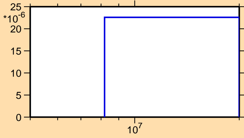
\sigma vs. E for ^{152}\text{Gd}(n,t)
