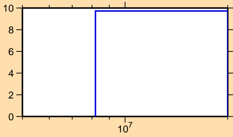
\Delta\sigma/\sigma vs. E for ^{152}\text{Gd}(n,2n)
