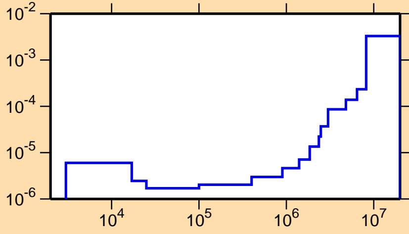
\sigma vs. E for ^{152}\text{Gd}(n,\alpha)
