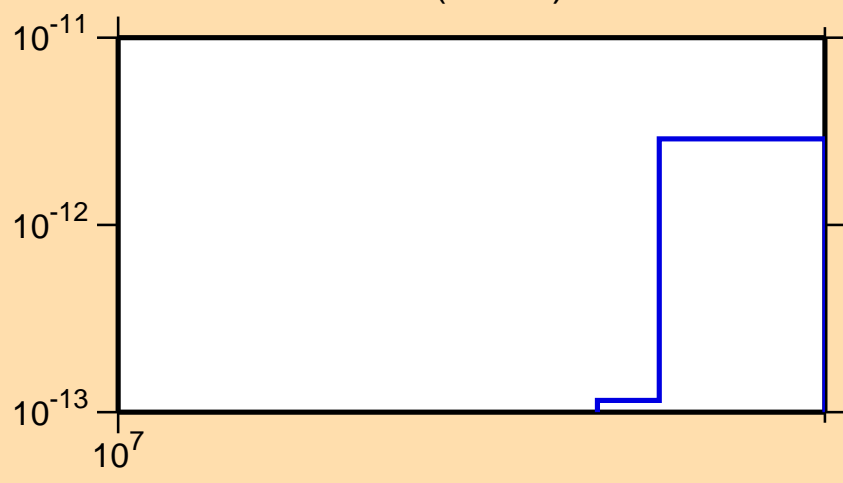
\sigma vs. E for ^{153}\text{Gd} (mt 45)
