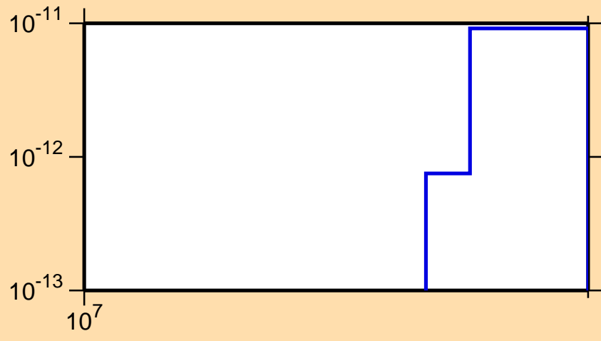
\sigma vs. E for ^{153}\text{Gd}(\text{mt117})
