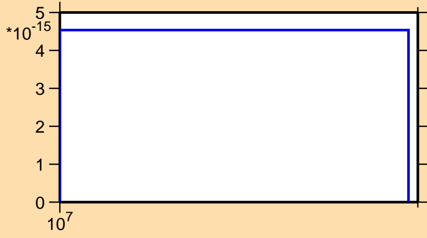
\sigma vs. E for ^{153}\text{Gd} (mt 34)
