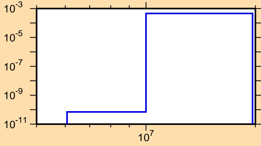
\sigma vs. E for ^{153}\text{Gd}(n,np)
