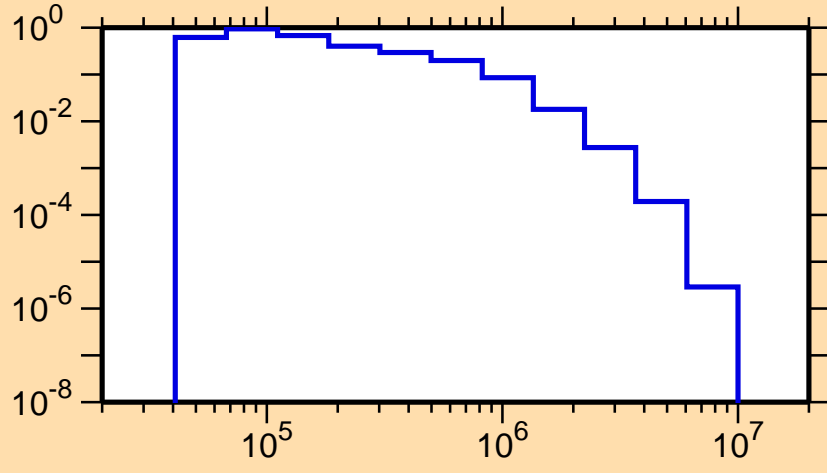
\sigma vs. E for ^{153}\text{Gd}(n,n_1)
