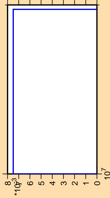
\Delta\sigma/\sigma vs. E for ^{153}\text{Gd}(n,\text{pt})
