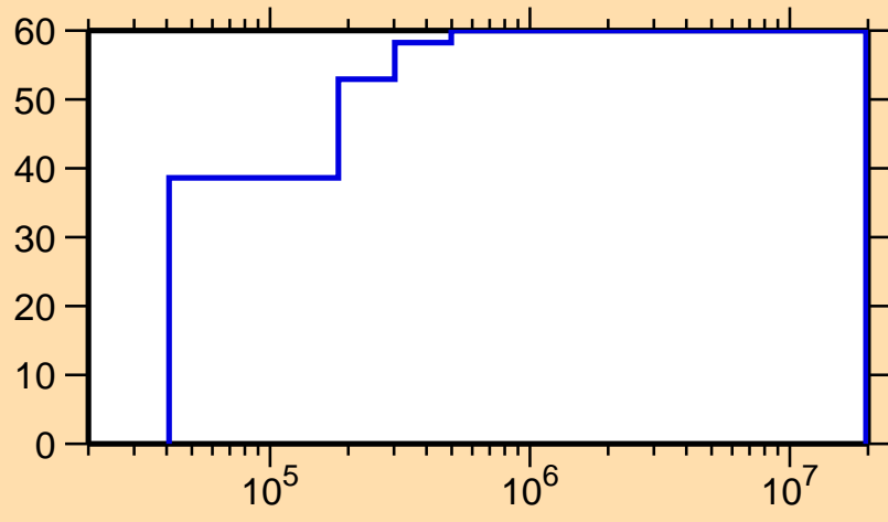
\Delta\sigma/\sigma vs. E for ^{153}\text{Gd}(n,n_1)
