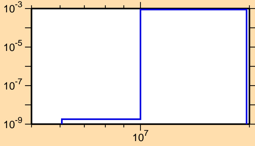
\sigma vs. E for ^{153}\text{Gd}(n,d)
