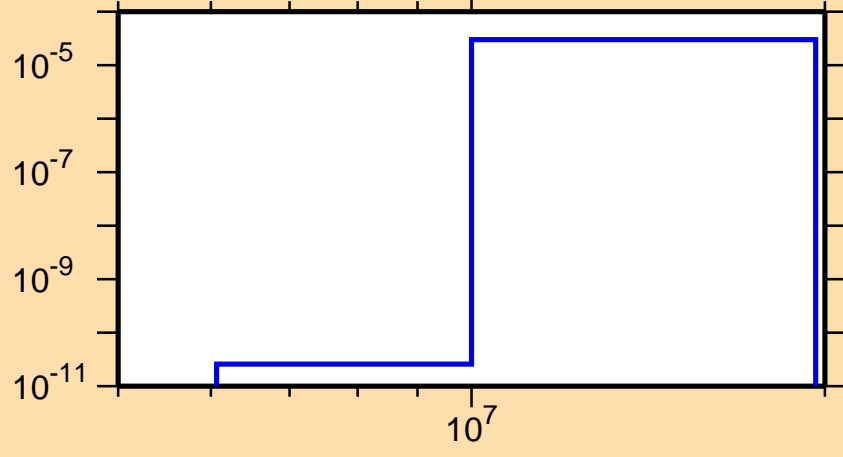
\sigma vs. E for ^{153}\text{Gd}(n,2n\alpha)
