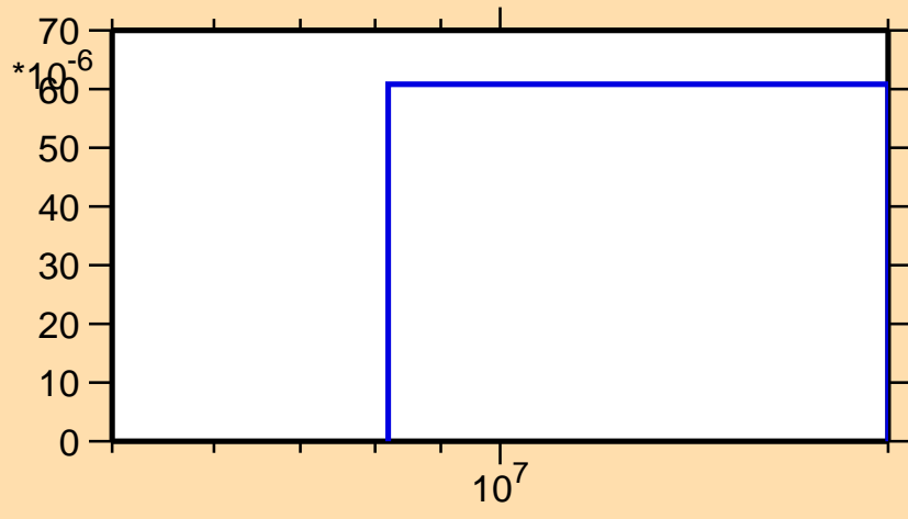
\sigma vs. E for ^{153}\text{Gd}(n,t)
