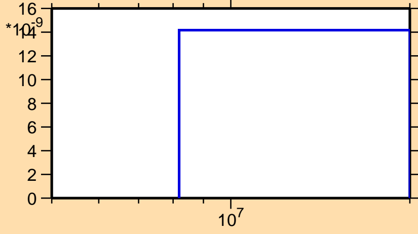
\sigma vs. E for ^{153}\text{Gd}(n,2np)
