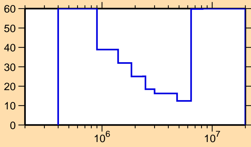
\Delta\sigma/\sigma vs. E for ^{153}\text{Gd}(n,n\text{cont.})
