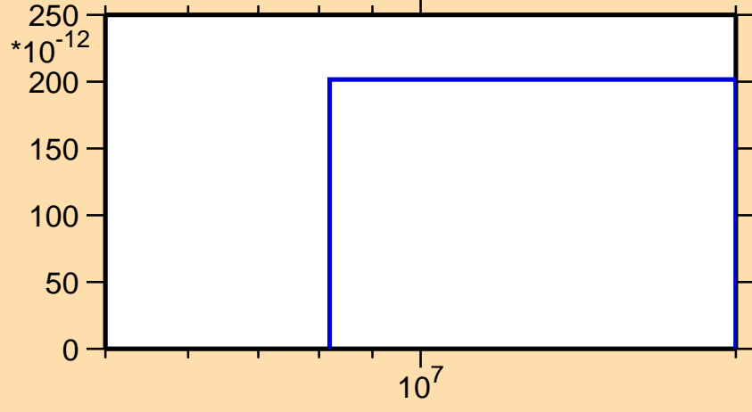
\sigma vs. E for ^{153}\text{Gd}(n,\text{He3})
