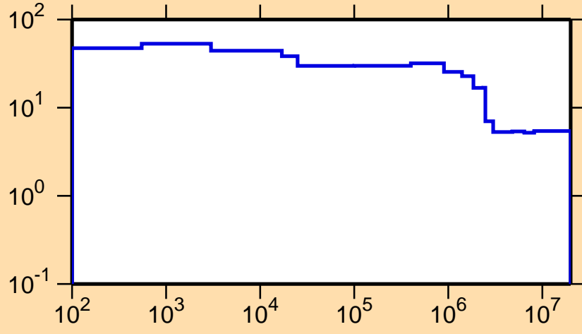
\Delta\sigma/\sigma vs. E for ^{153}\text{Gd}(n,\text{nonel.})
