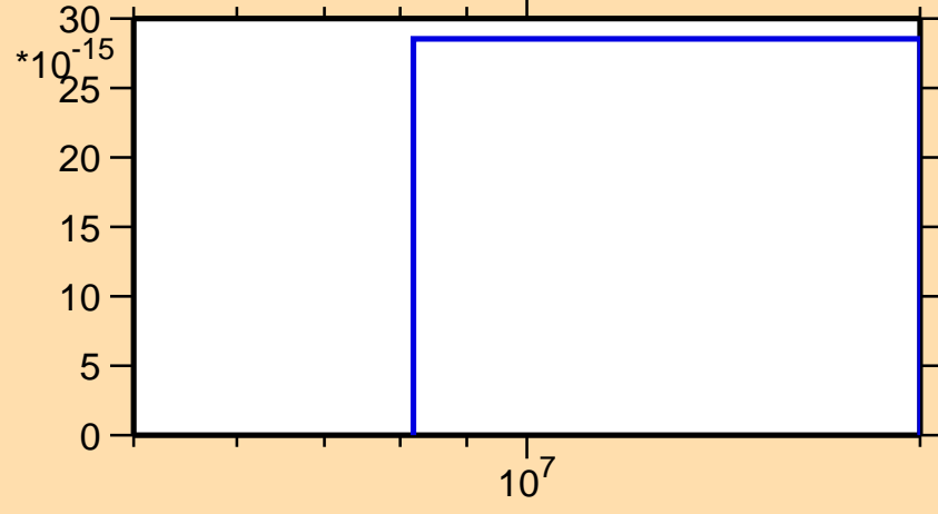
\sigma vs. E for ^{153}\text{Gd} (mt 45)
