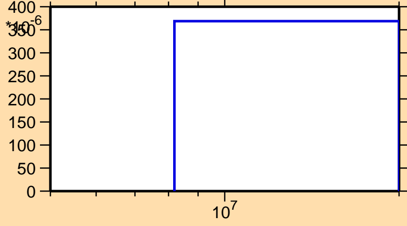
\sigma vs. E for ^{153}\text{Gd}(n,np)
