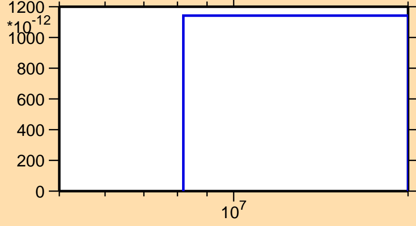
\sigma vs. E for ^{153}\text{Gd}(n,p\alpha)
