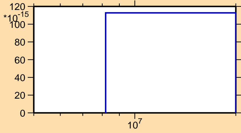
\sigma vs. E for ^{153}\text{Gd}(\text{mt117})
