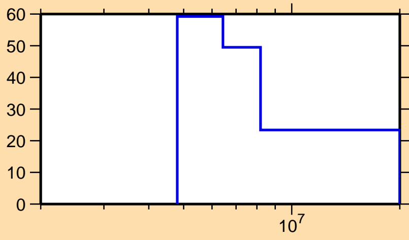
\Delta\sigma/\sigma vs. E for ^{153}\text{Gd}(n,2n)
