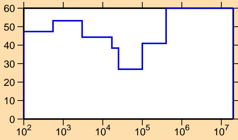
\Delta\sigma/\sigma vs. E for ^{153}\text{Gd}(n,\gamma)
