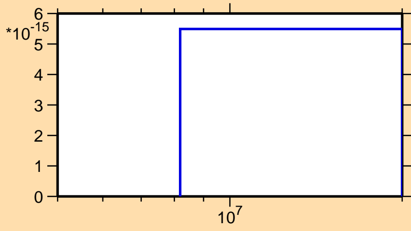
\sigma vs. E for ^{153}\text{Gd} (mt 34)
