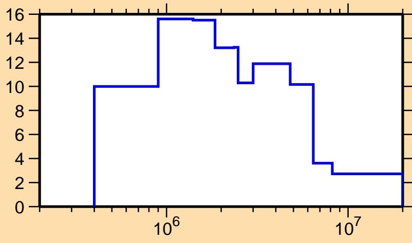
\Delta\sigma/\sigma vs. E for ^{153}\text{Gd}(n,\text{tot.})
