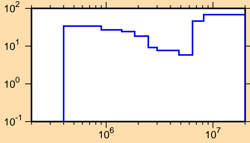
\Delta\sigma/\sigma vs. E for ^{153}\text{Gd}(n,\text{inel.})
