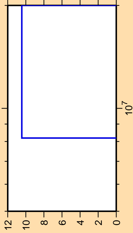
\Delta\sigma/\sigma vs. E for ^{153}\text{Gd}(n,3n\alpha)
