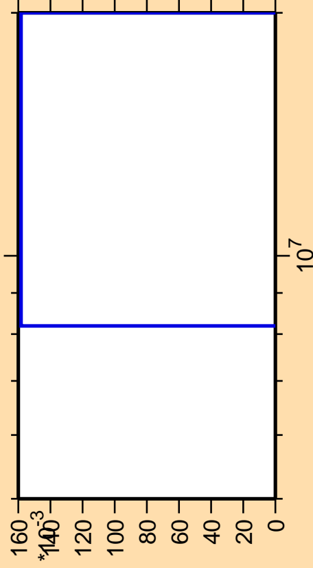
\Delta\sigma/\sigma vs. E for ^{153}\text{Gd} (mt 45)
