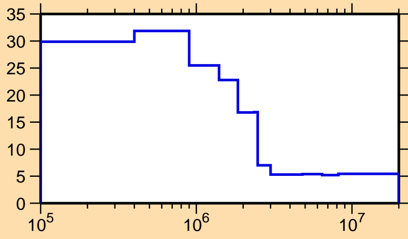
\Delta\sigma/\sigma vs. E for ^{153}\text{Gd}(n,\text{nonel.})
