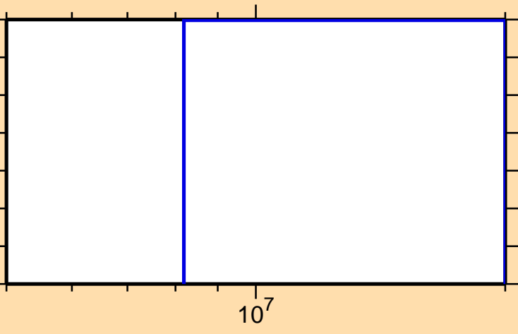
\sigma vs. E for ^{153}\text{Gd}(n,3n)
