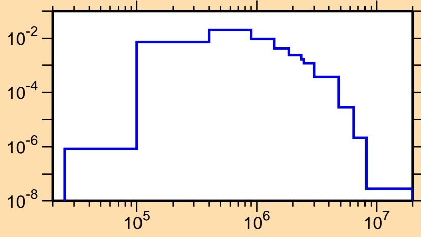
\sigma vs. E for ^{153}\text{Gd}(n,n_3)
