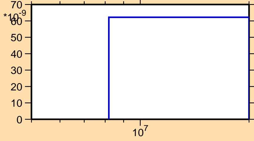
\sigma vs. E for ^{153}\text{Gd}(n,nd)
