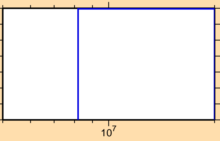
\sigma vs. E for ^{153}\text{Gd}(n,\text{pt})
