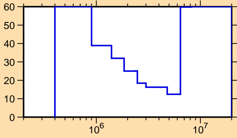
\Delta\sigma/\sigma vs. E for ^{153}\text{Gd}(n,n\text{cont.})
