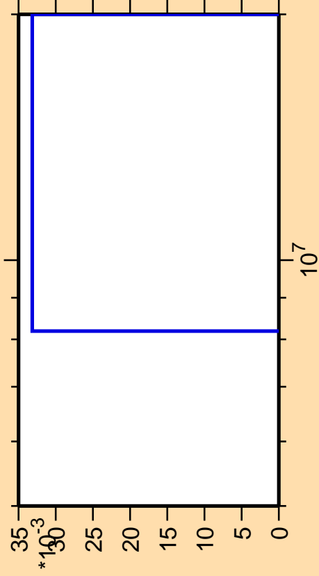
\Delta\sigma/\sigma vs. E for ^{153}\text{Gd} (mt 34)
