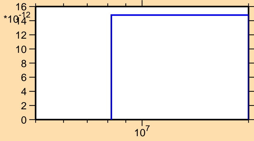
\sigma vs. E for ^{153}\text{Gd}(n,3n\alpha)
