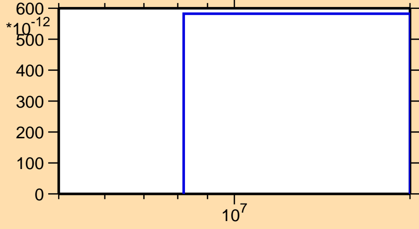
\sigma vs. E for ^{153}\text{Gd}(n,nt)
