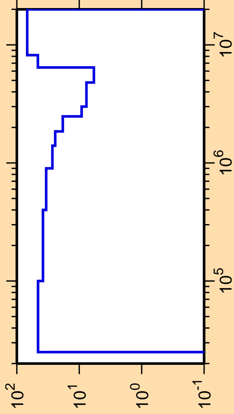
\Delta\sigma/\sigma vs. E for ^{153}\text{Gd}(n,\text{inel.})
