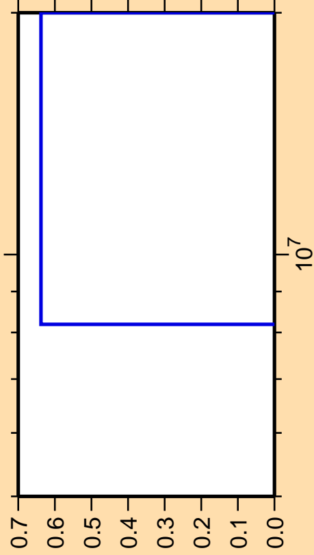
\Delta\sigma/\sigma vs. E for ^{153}\text{Gd}(\text{mt117})
