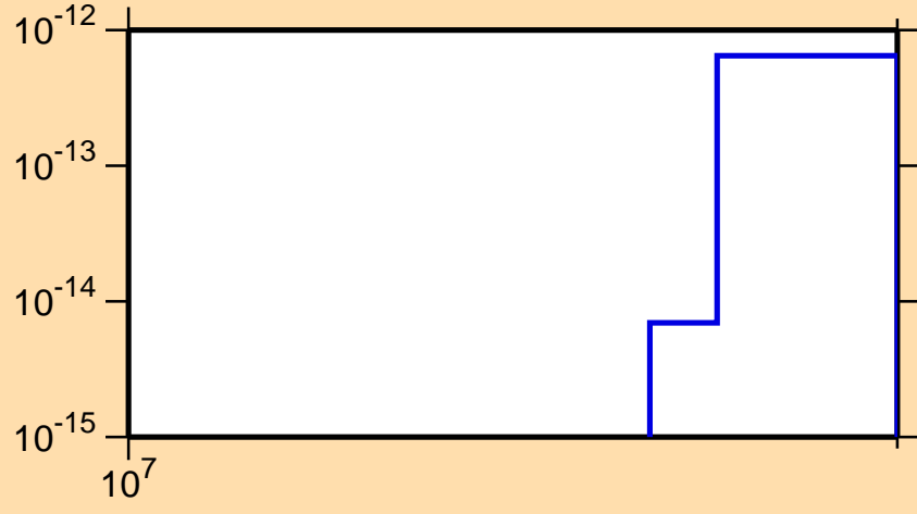
\sigma vs. E for ^{154}\text{Gd}(\text{mt117})
