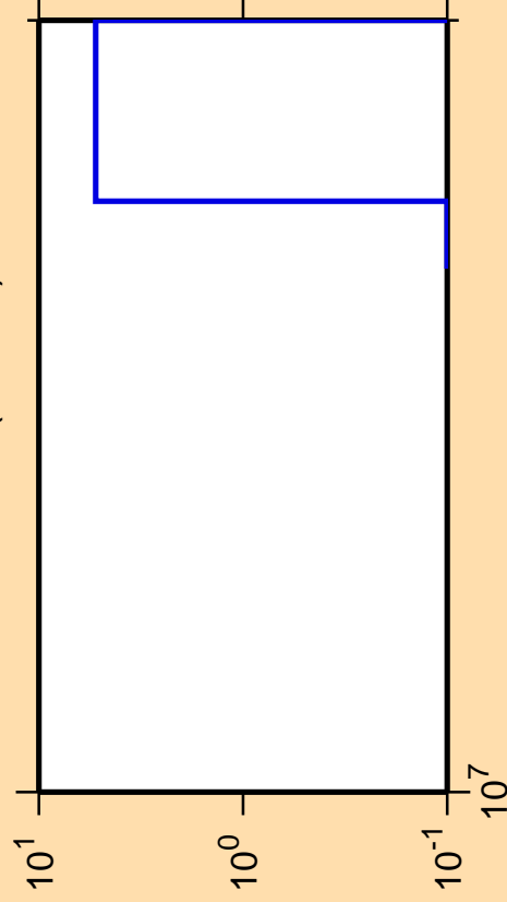
\Delta\sigma/\sigma vs. E for ^{154}\text{Gd}(\text{mt117})
