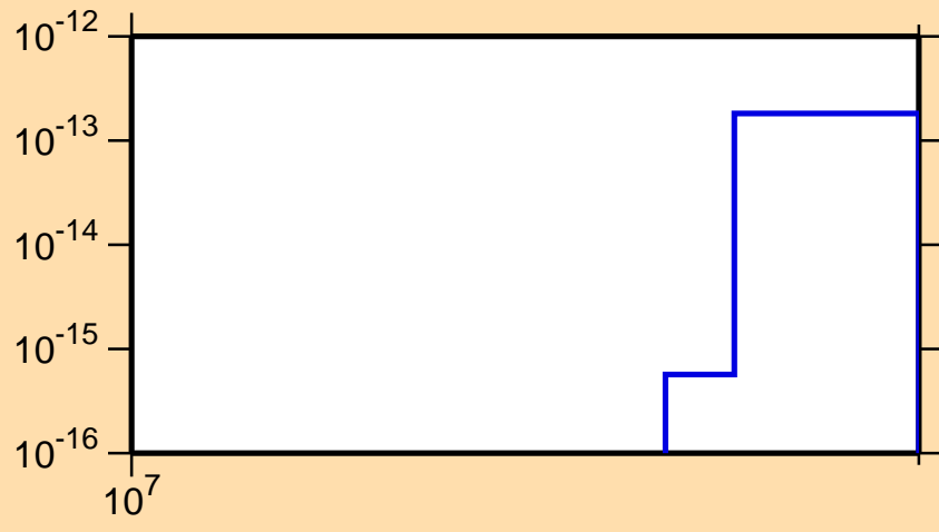
\sigma vs. E for ^{154}\text{Gd} (mt 45)
