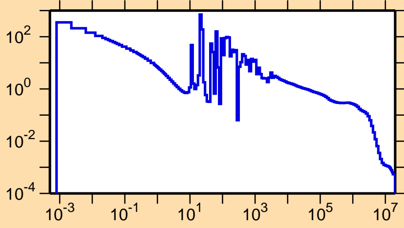
\sigma vs. E for ^{154}\text{Gd}(n,\gamma)
