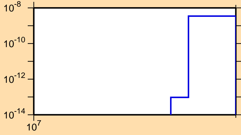
\sigma vs. E for ^{154}\text{Gd}(n,nt)
