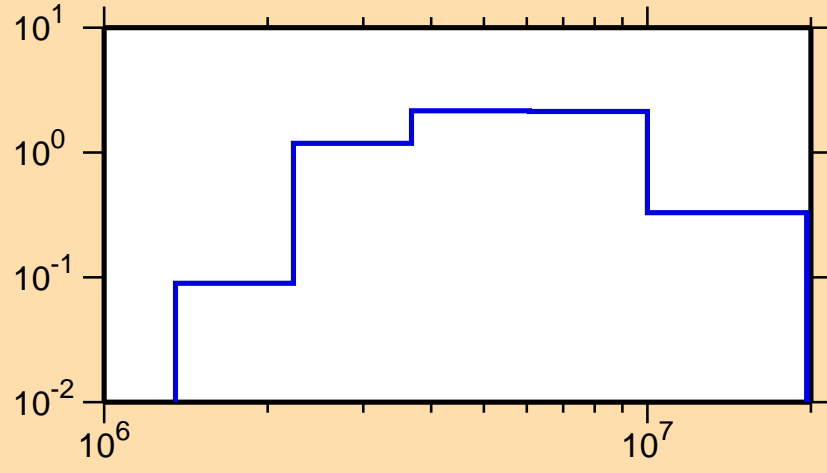
\sigma vs. E for ^{154}\text{Gd}(n,n\text{cont.})
