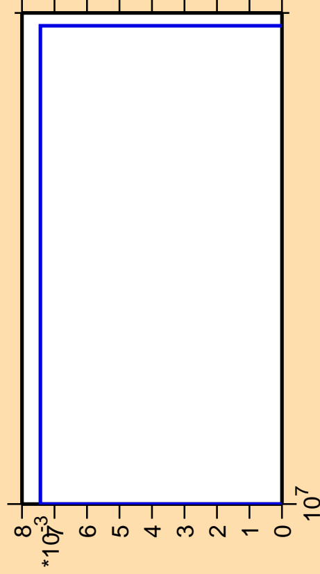
\Delta\sigma/\sigma vs. E for ^{154}\text{Gd} (mt 45)
