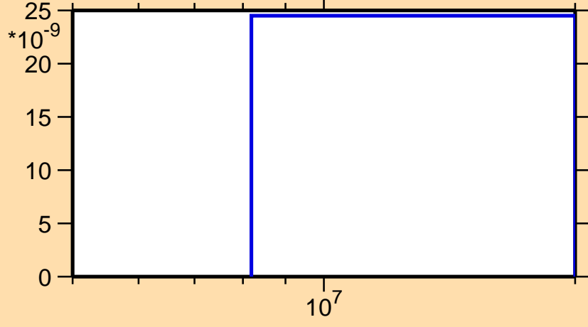
\sigma vs. E for ^{155}\text{Gd}(n,nd)
