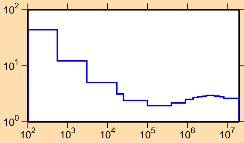
\sigma vs. E for ^{155}\text{Gd}(n,\text{nonel.})
