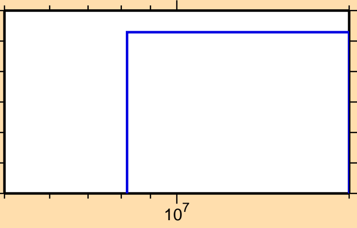
\sigma vs. E for ^{155}\text{Gd}(n,np)
