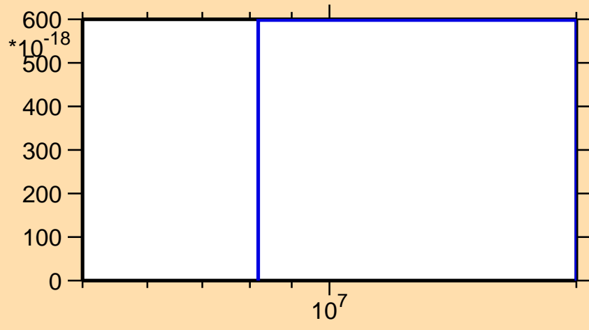
\sigma vs. E for ^{155}\text{Gd}(n,3n\alpha)
