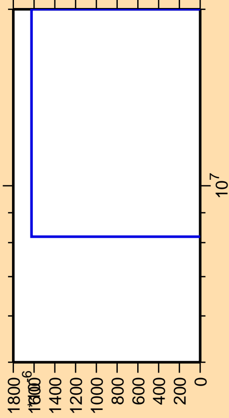
\Delta\sigma/\sigma vs. E for ^{155}\text{Gd}(n,3n\alpha)
