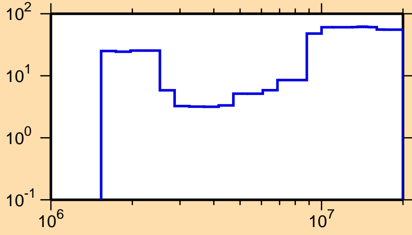
\Delta\sigma/\sigma vs. E for ^{156}\text{Gd}(n,n\text{cont.})
