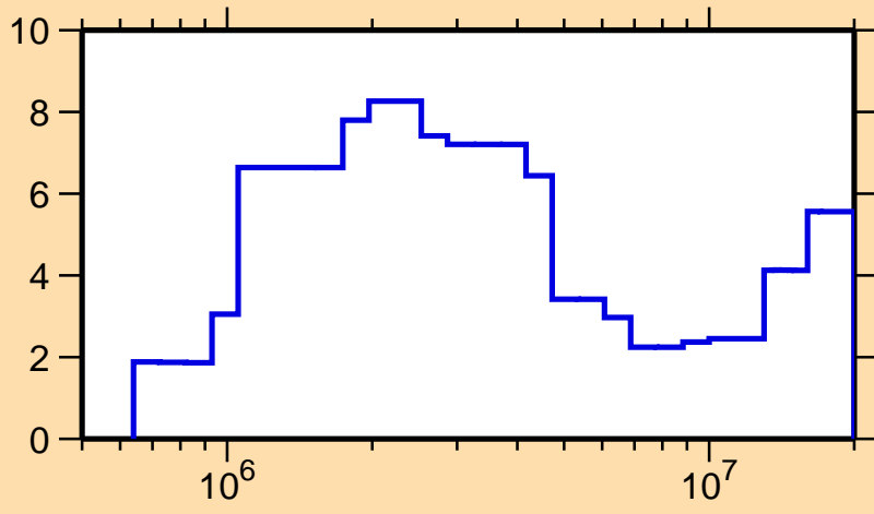
\Delta\sigma/\sigma vs. E for ^{157}\text{Gd}(n,tot.)
