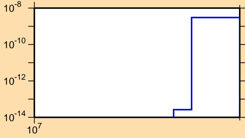
\sigma vs. E for ^{157}\text{Gd}(n,nt)
