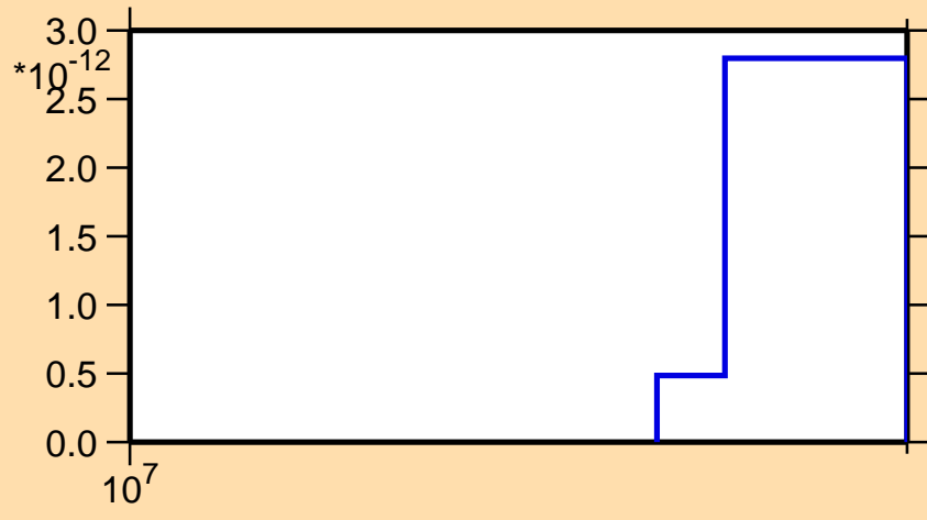
\sigma vs. E for ^{157}\text{Gd}(n,p\alpha)
