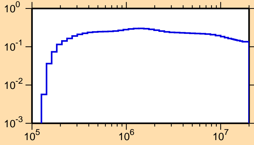
\sigma vs. E for ^{157}\text{Gd}(n,n_4)
