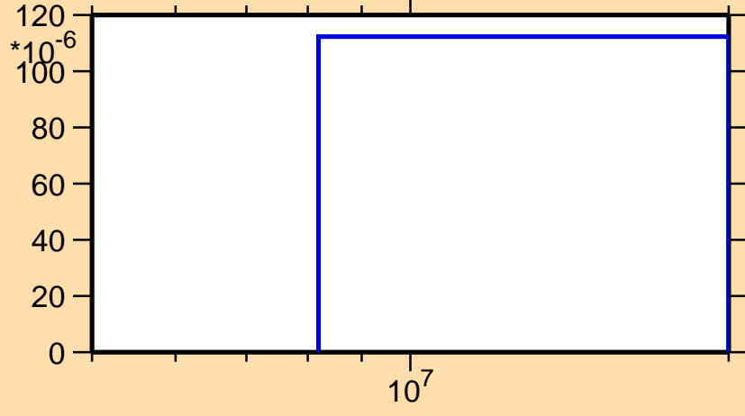
\sigma vs. E for ^{157}\text{Gd}(n,np)
