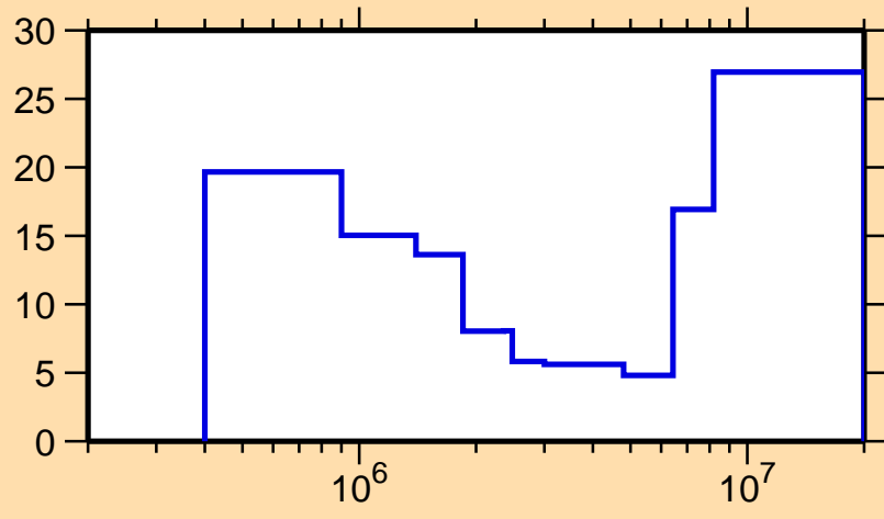
\Delta\sigma/\sigma vs. E for ^{157}\text{Gd}(n,n\text{cont.})
