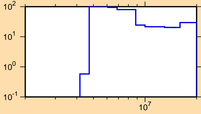
\Delta\sigma/\sigma vs. E for ^{158}\text{Gd}(n,p)
