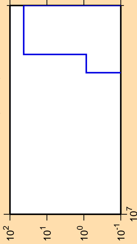
\Delta\sigma/\sigma vs. E for ^{158}\text{Gd}(n,\text{He3})
