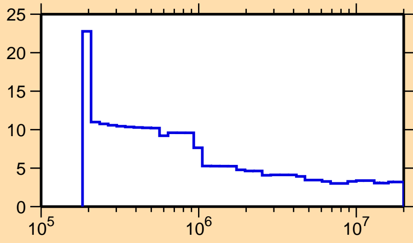
\Delta\sigma/\sigma vs. E for ^{158}\text{Gd}(n,\text{nonel.})
