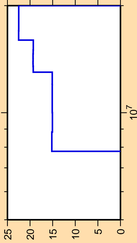
\Delta\sigma/\sigma vs. E for ^{158}\text{Gd}(n,n_1)
