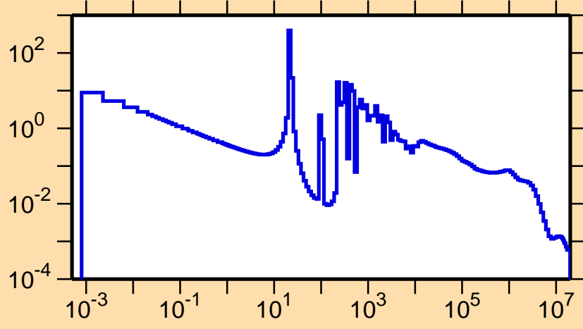
\sigma vs. E for ^{158}\text{Gd}(n,\gamma)
