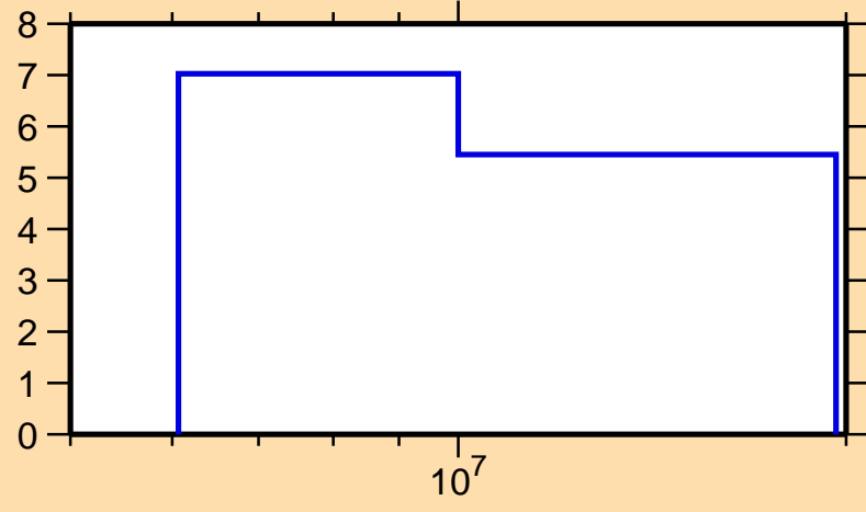
\Delta\sigma/\sigma vs. E for ^{158}\text{Gd}(n,2n)
