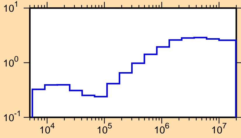
\sigma vs. E for ^{158}\text{Gd}(n,\text{nonel.})
