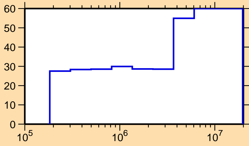
\Delta\sigma/\sigma vs. E for ^{158}\text{Gd}(n,\gamma)
