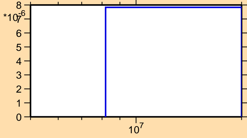
\sigma vs. E for ^{158}\text{Gd}(n,t)
