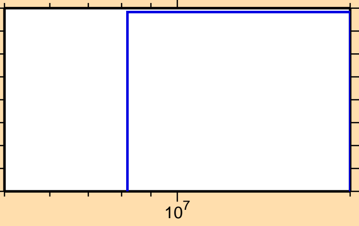
\sigma vs. E for ^{158}\text{Gd}(n,t)
