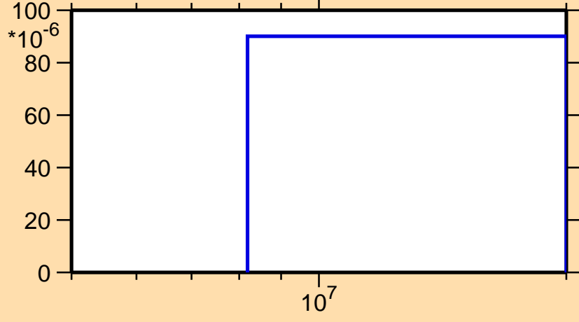
\sigma vs. E for ^{158}\text{Gd}(n,np)
