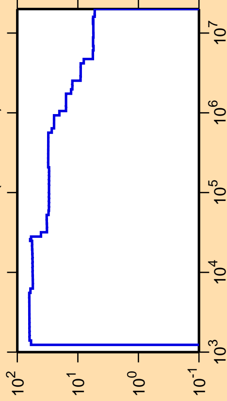
\Delta\sigma/\sigma vs. E for ^{159}\text{Gd}(n,\text{nonel.})
