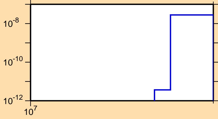
\sigma vs. E for ^{159}\text{Gd}(n,nt)
