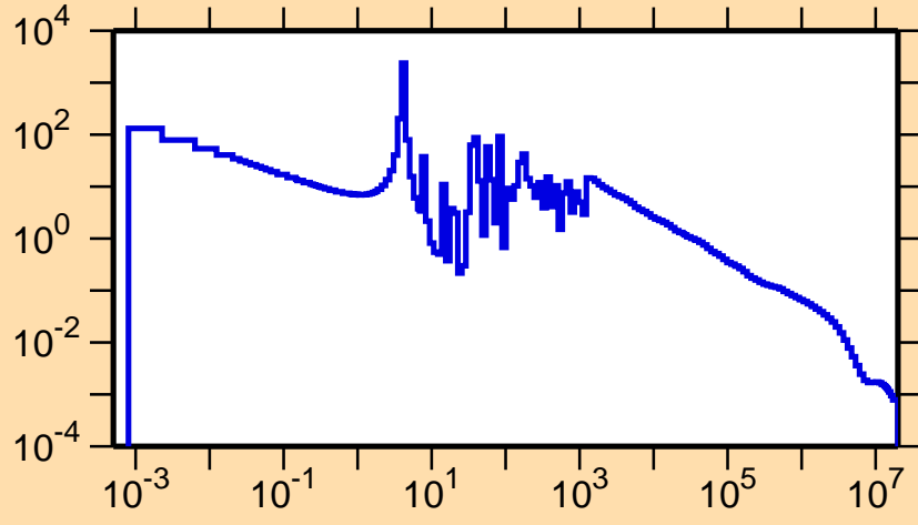
\sigma vs. E for ^{159}\text{Gd}(n,\gamma)
