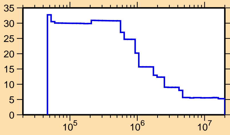
\Delta\sigma/\sigma vs. E for ^{159}\text{Gd}(n,\text{nonel.})
