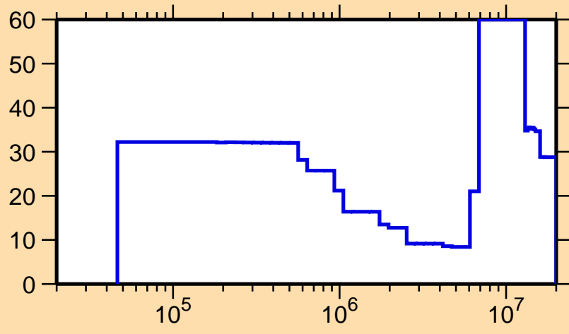
\Delta\sigma/\sigma vs. E for ^{159}\text{Gd}(n,\text{inel.})
