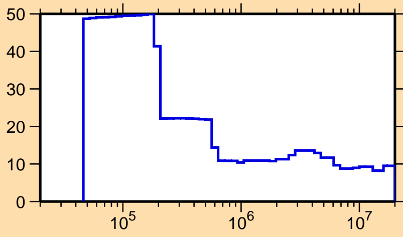
\Delta\sigma/\sigma vs. E for ^{159}\text{Gd}(n,\text{el.})
