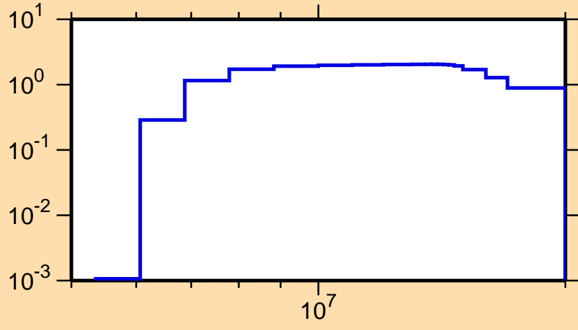
\sigma vs. E for ^{159}\text{Gd}(n,2n)
