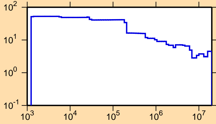
\Delta\sigma/\sigma vs. E for ^{159}\text{Gd}(n,\text{tot.})
