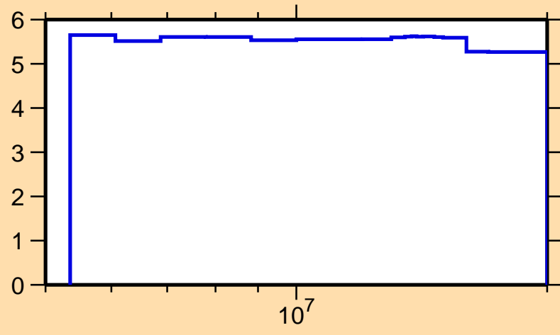
\Delta\sigma/\sigma vs. E for ^{159}\text{Gd}(n,\text{nonel.})
