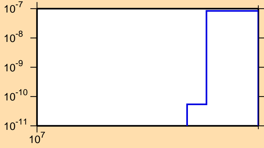
\sigma vs. E for ^{159}\text{Gd}(n,2np)
