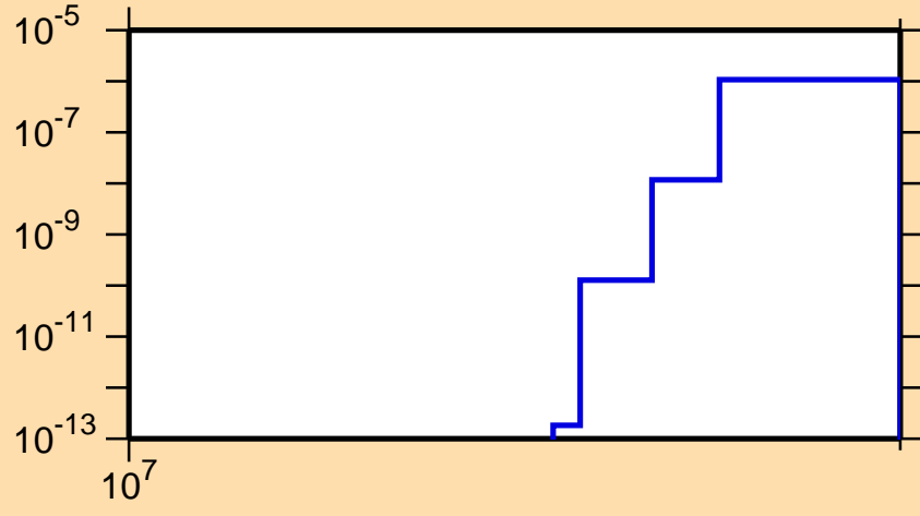
\sigma vs. E for ^{159}\text{Gd}(n,\text{nd})
