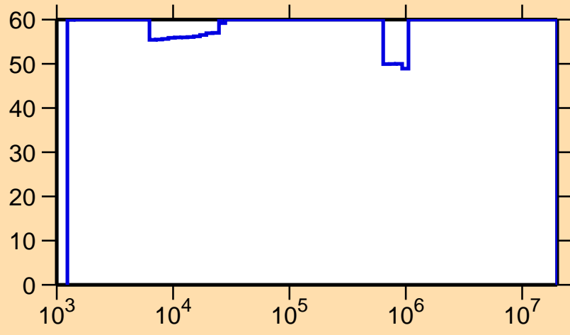
\Delta\sigma/\sigma vs. E for ^{159}\text{Gd}(n,\gamma)
