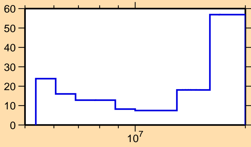
\Delta\sigma/\sigma vs. E for ^{159}\text{Gd}(n,2n)
