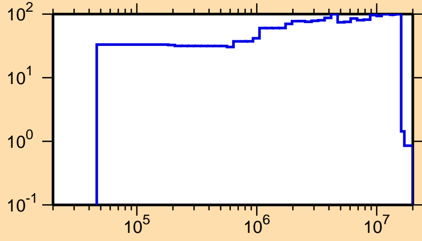
\Delta\sigma/\sigma vs. E for ^{159}\text{Gd}(n,n_1)
