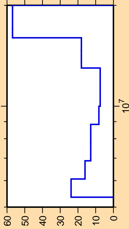
\Delta\sigma/\sigma vs. E for ^{159}\text{Gd}(n,2n)
