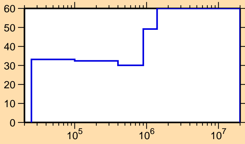
\Delta\sigma/\sigma vs. E for ^{159}\text{Gd}(n,n_1)
