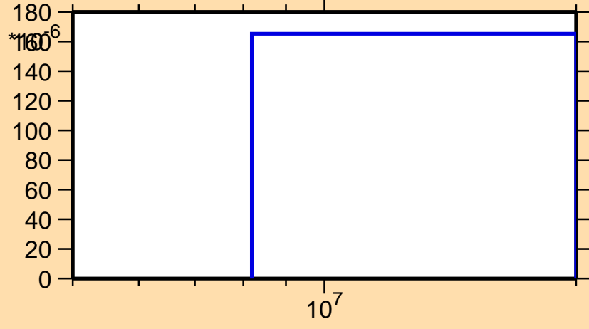
\sigma vs. E for ^{159}\text{Gd}(n,d)
