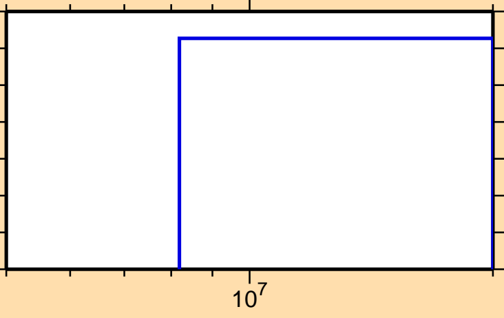
\sigma vs. E for ^{159}\text{Gd}(n,\text{He3})
