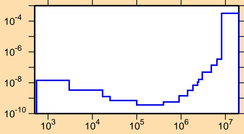
\sigma vs. E for ^{159}\text{Gd}(n,\alpha)
