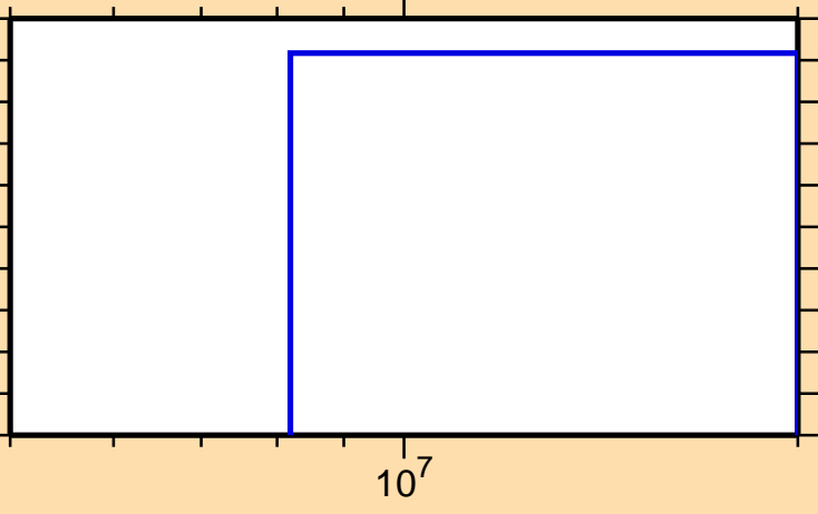
\sigma vs. E for ^{159}\text{Gd}(n,t)
