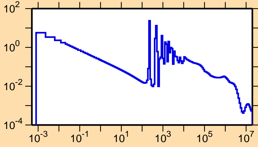
\sigma vs. E for ^{160}\text{Gd}(n,\gamma)
