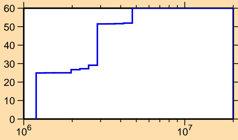
\Delta\sigma/\sigma vs. E for ^{160}\text{Gd}(n,\gamma)
