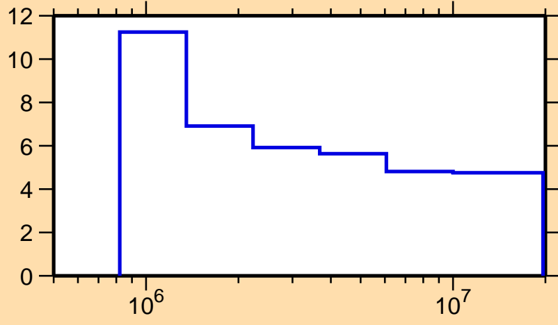
\Delta\sigma/\sigma vs. E for ^{160}\text{Gd}(n,\text{nonel.})
