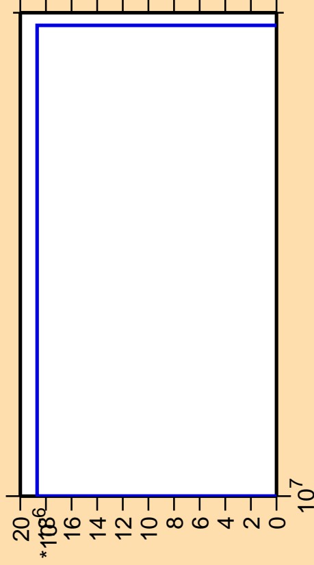
\Delta\sigma/\sigma vs. E for ^{160}\text{Gd}(n,3n\alpha)
