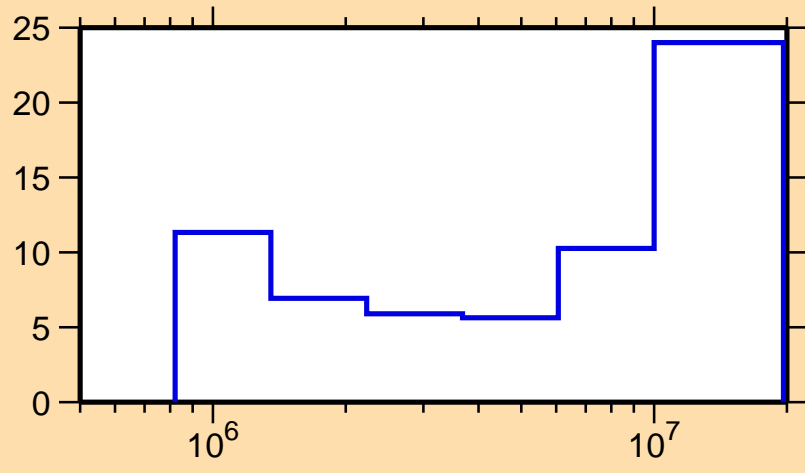
\Delta\sigma/\sigma vs. E for ^{160}\text{Gd}(n,\text{inel.})
