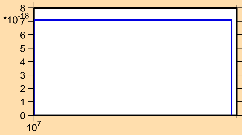
\sigma vs. E for ^{160}\text{Gd}(n,3n\alpha)
