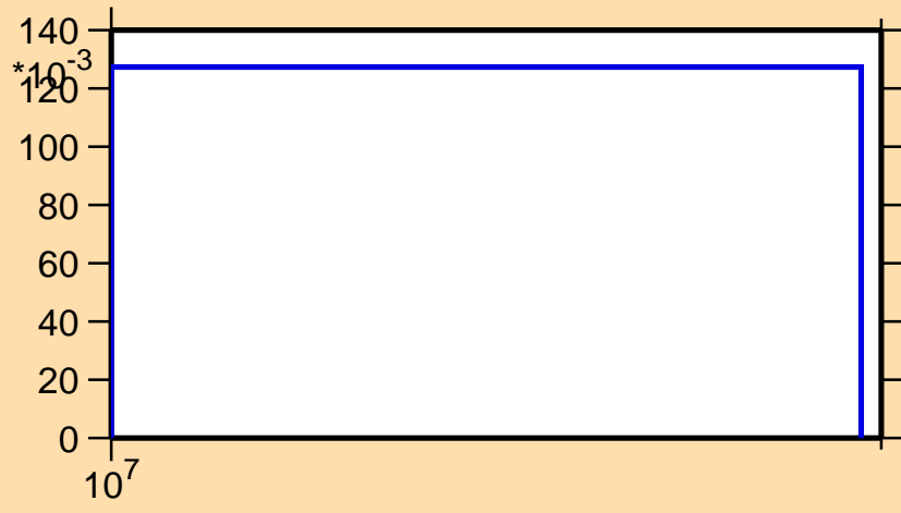
\sigma vs. E for ^{160}\text{Gd}(n,3n)
