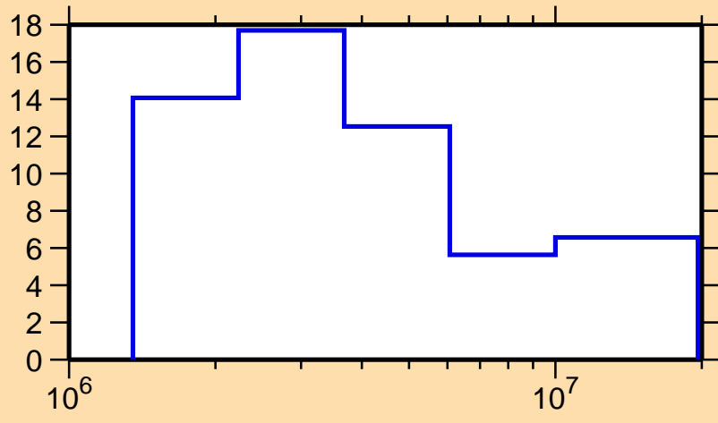
\Delta\sigma/\sigma vs. E for ^{160}\text{Gd}(n,\text{el.})
