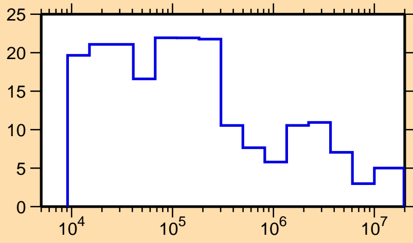
\Delta\sigma/\sigma vs. E for ^{160}\text{Gd}(n,\text{tot.})
