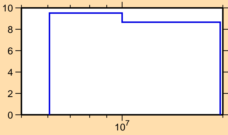
\Delta\sigma/\sigma vs. E for ^{160}\text{Gd}(n,2n)
