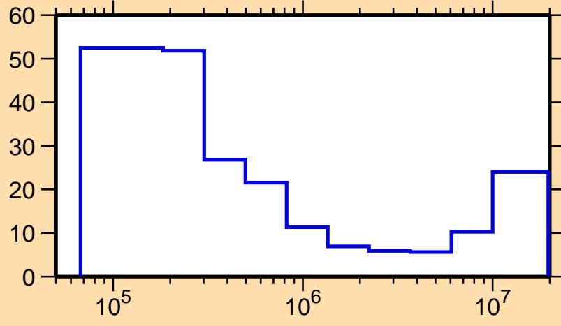
\Delta\sigma/\sigma vs. E for ^{160}\text{Gd}(n,\text{inel.})
