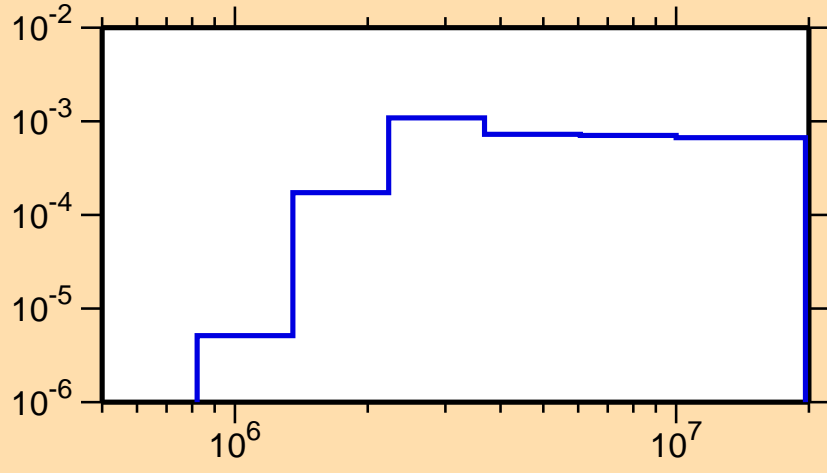
\sigma vs. E for ^{160}\text{Gd}(n,n_4)
