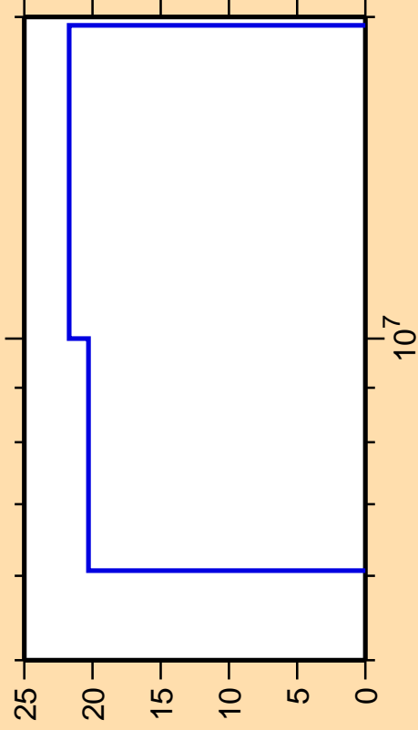
\Delta\sigma/\sigma vs. E for ^{160}\text{Gd}(n,n_1)
