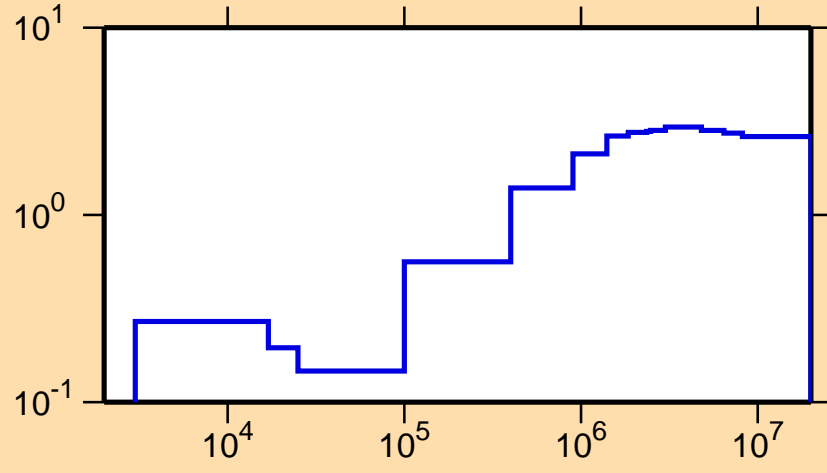
\sigma vs. E for ^{160}\text{Gd}(n,\text{nonel.})
