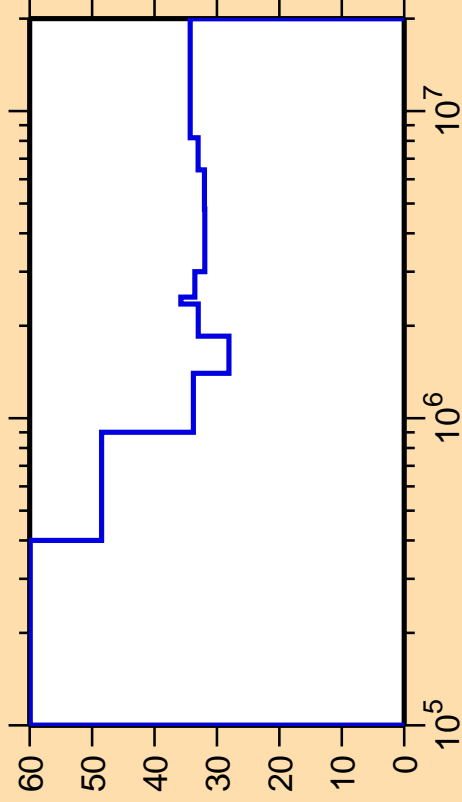
\Delta\sigma/\sigma vs. E for ^{160}\text{Gd}(n,n_2)
