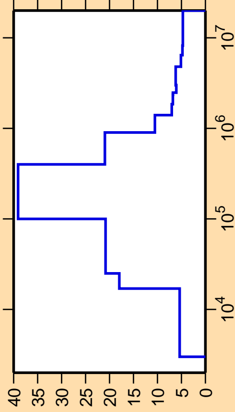
\Delta\sigma/\sigma vs. E for ^{160}\text{Gd}(n,\text{nonel.})
