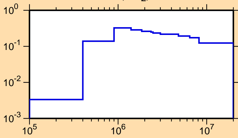
\sigma vs. E for ^{160}\text{Gd}(n,n_2)
