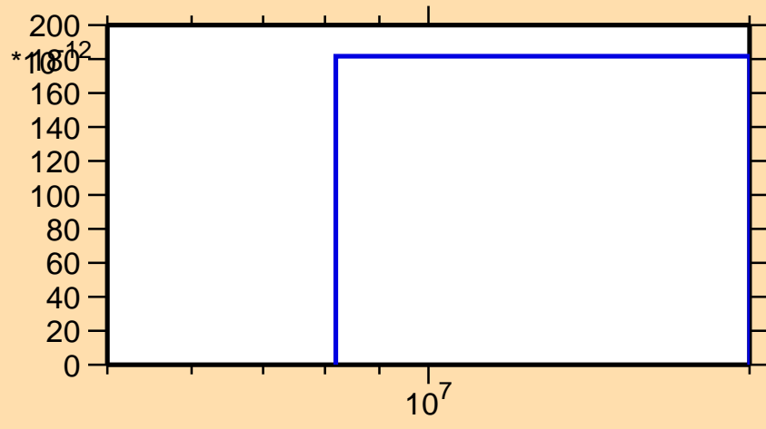
\sigma vs. E for ^{160}\text{Gd}(n,nt)
