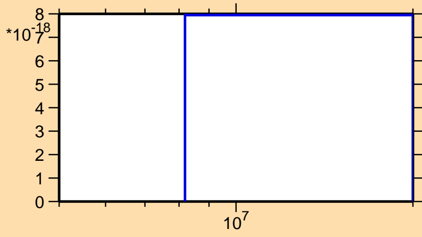
\sigma vs. E for ^{160}\text{Gd}(n,3n\alpha)
