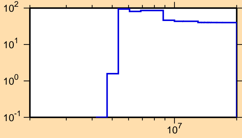
\Delta\sigma/\sigma vs. E for ^{161}\text{Gd}(n,p)
