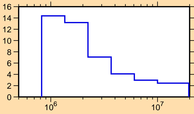
\Delta\sigma/\sigma vs. E for ^{161}\text{Gd}(n,n\text{onel.})
