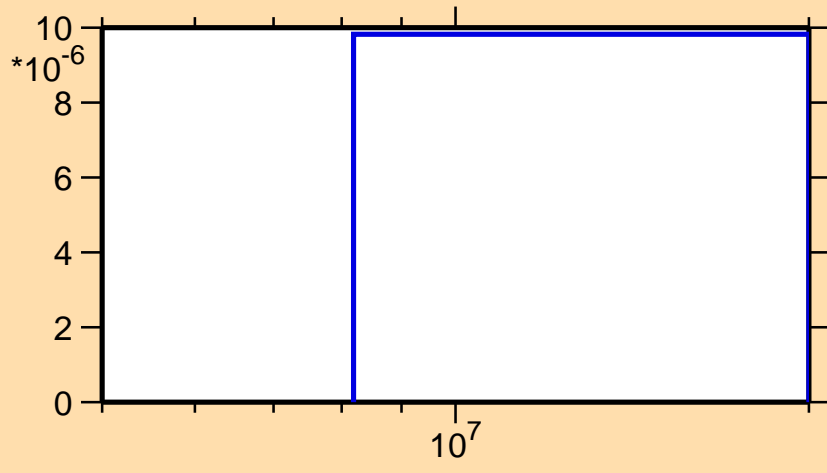
\sigma vs. E for ^{161}\text{Gd}(n,t)
