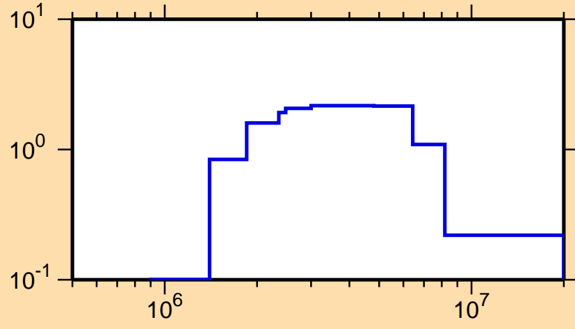
\sigma vs. E for ^{161}\text{Gd}(n,n\text{cont.})
