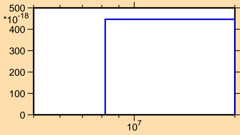
\sigma vs. E for ^{161}\text{Gd}(n,\text{He3})
