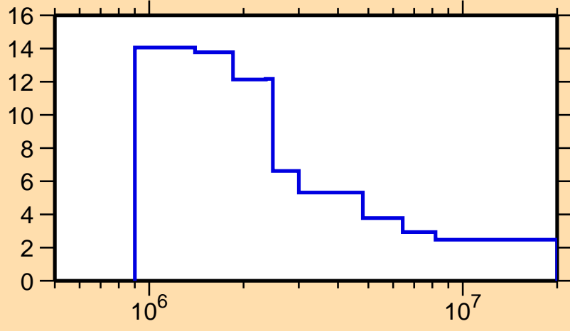
\Delta\sigma/\sigma vs. E for ^{161}\text{Gd}(n,n\text{nonel.})
