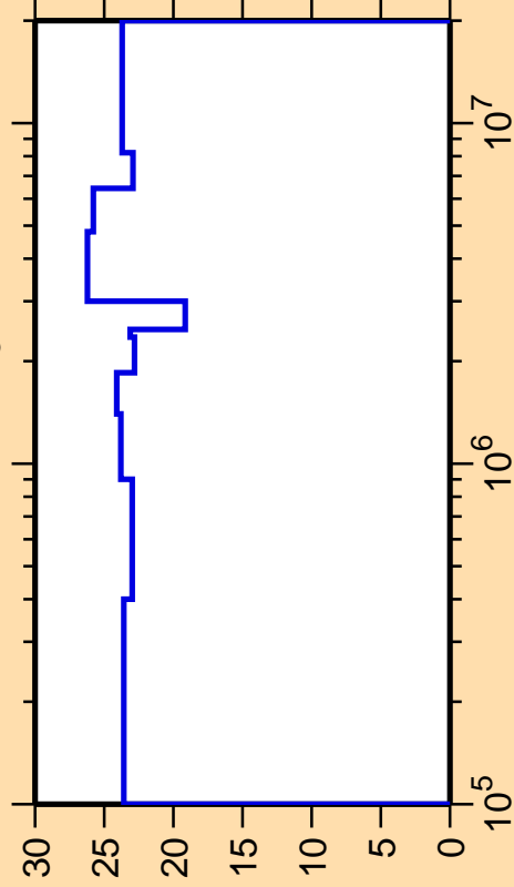
\Delta\sigma/\sigma vs. E for ^{161}\text{Gd}(n,n_3)
