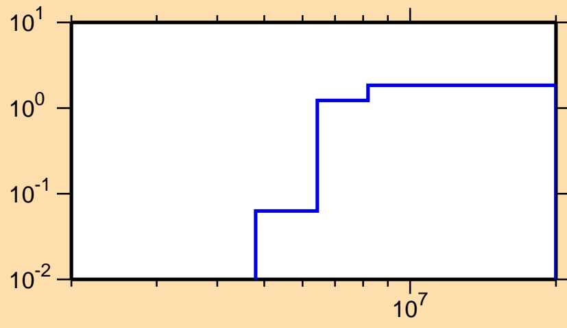
\sigma vs. E for ^{161}\text{Gd}(n,2n)
