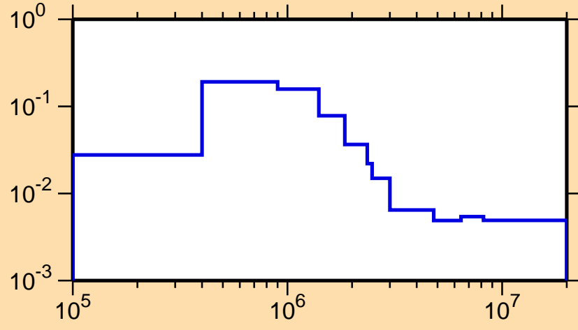
\sigma vs. E for ^{161}\text{Gd}(n,n_3)
