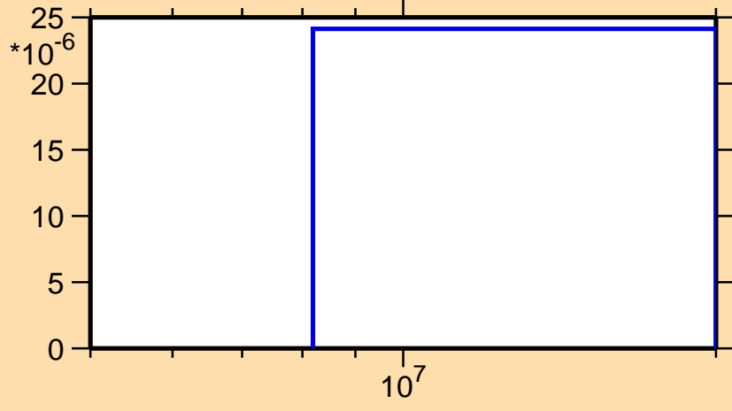
\sigma vs. E for ^{161}\text{Gd}(n,np)
