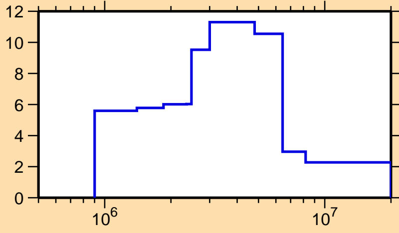
\Delta\sigma/\sigma vs. E for ^{161}\text{Gd}(n,\text{el.})
