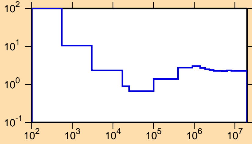
\sigma vs. E for ^{161}\text{Gd}(n,\text{nonel.})
