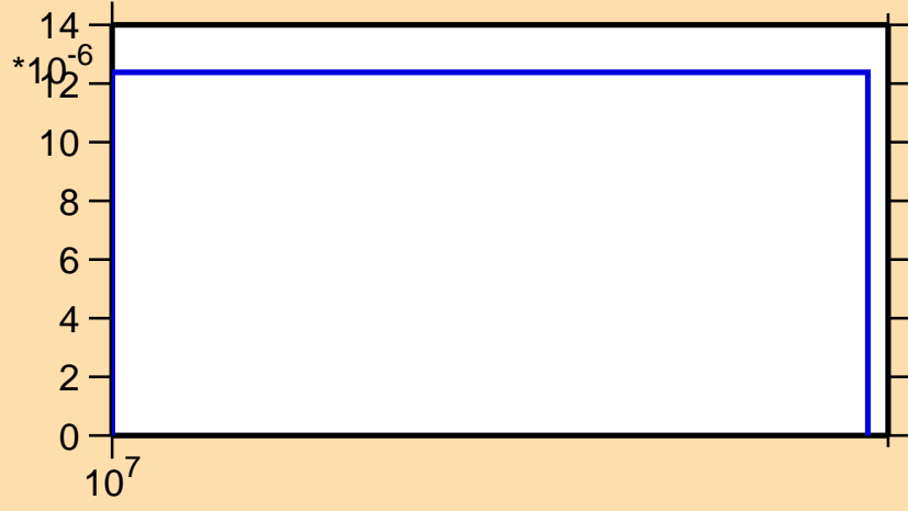
\sigma vs. E for ^{162}\text{Gd}(n,np)
