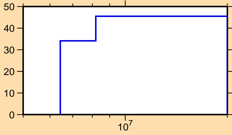
\Delta\sigma/\sigma vs. E for ^{162}\text{Gd}(n,ncont.)
