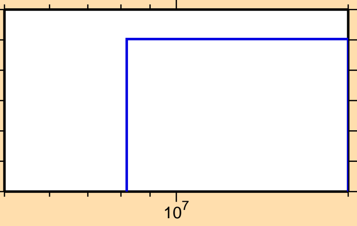
\sigma vs. E for ^{162}\text{Gd}(n,np)
