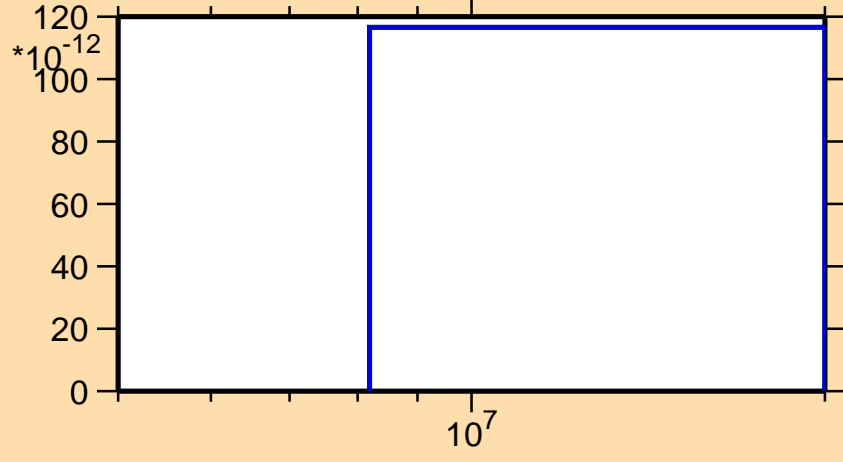
\sigma vs. E for ^{162}\text{Gd}(n,nd)
