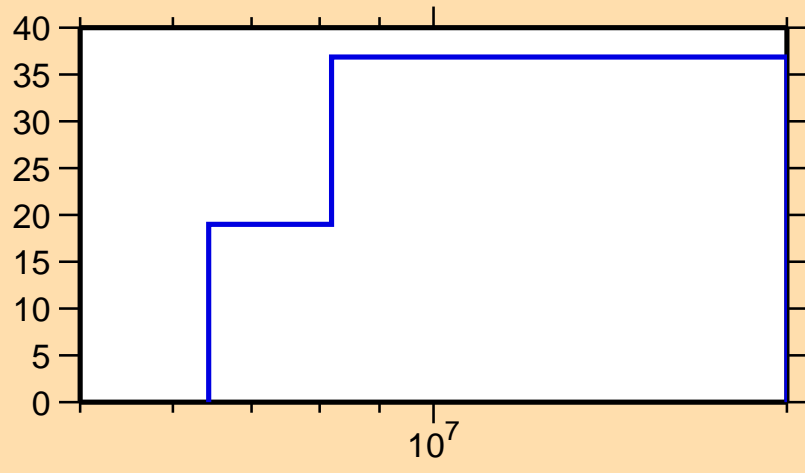
\Delta\sigma/\sigma vs. E for ^{162}\text{Gd}(n,p)
