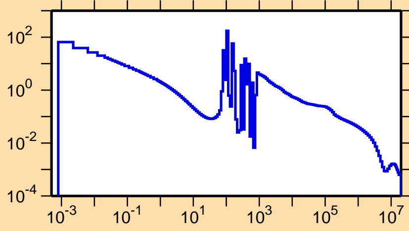
\sigma vs. E for ^{163}\text{Gd}(n,\gamma)
