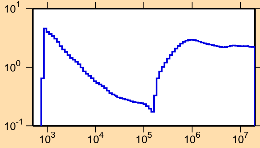
\sigma vs. E for ^{163}\text{Gd}(n,\text{nonel.})
