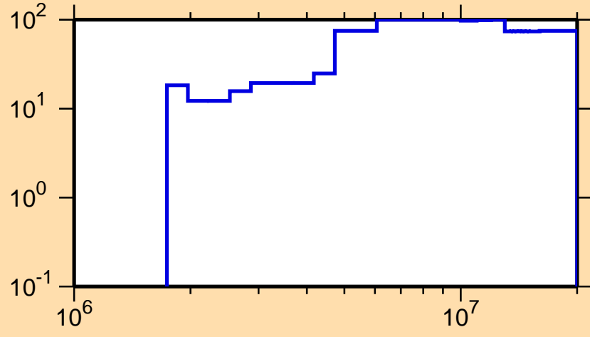
\Delta\sigma/\sigma vs. E for ^{163}\text{Gd}(n,n\text{cont.})
