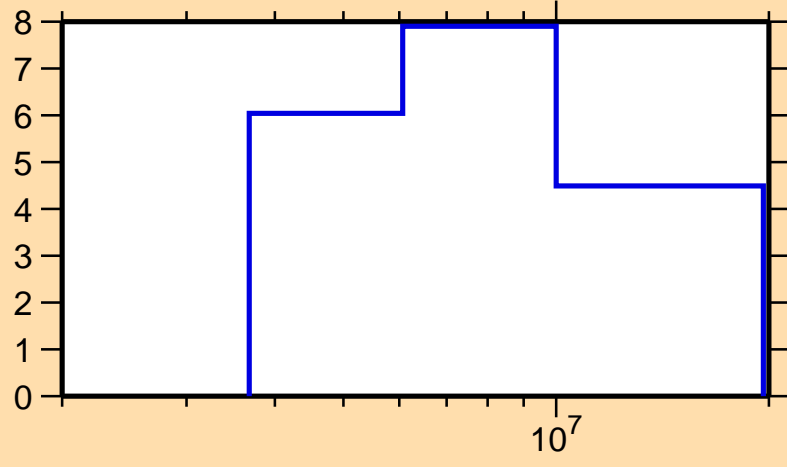
\Delta\sigma/\sigma vs. E for ^{163}\text{Gd}(n,\text{tot.})
