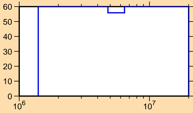
\Delta\sigma/\sigma vs. E for ^{163}\text{Gd}(n,\gamma)
