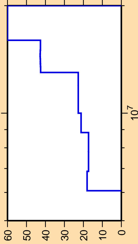
\Delta\sigma/\sigma vs. E for ^{164}\text{Gd}(n,2n)
