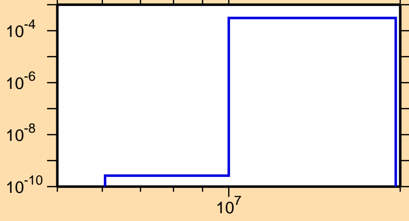
\sigma vs. E for ^{164}\text{Gd}(n,p)
