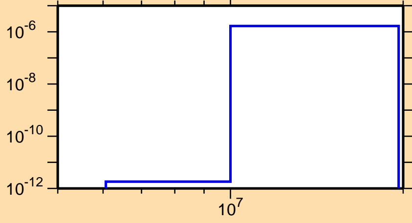
\sigma vs. E for ^{164}\text{Gd}(n,n\alpha)
