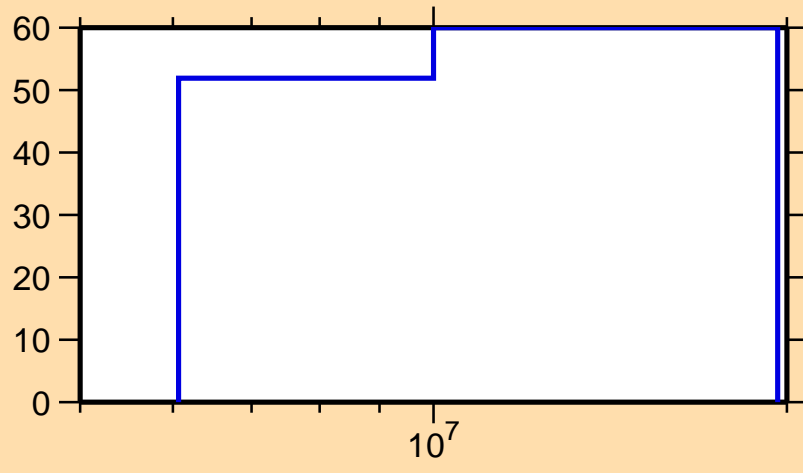
\Delta\sigma/\sigma vs. E for ^{164}\text{Gd}(n,\gamma)
