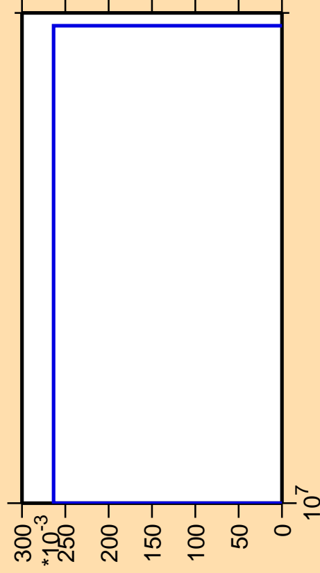
\Delta\sigma/\sigma vs. E for ^{164}\text{Gd}(n,2np)
