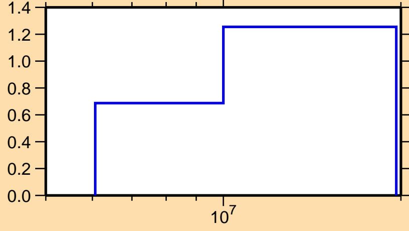
\sigma vs. E for ^{164}\text{Gd}(n,2n)
