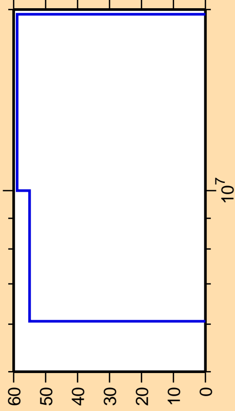
\Delta\sigma/\sigma vs. E for ^{164}\text{Gd}(n,n_1)
