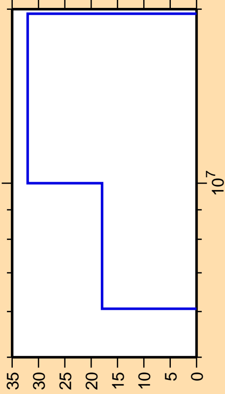
\Delta\sigma/\sigma vs. E for ^{164}\text{Gd}(n,2n)
