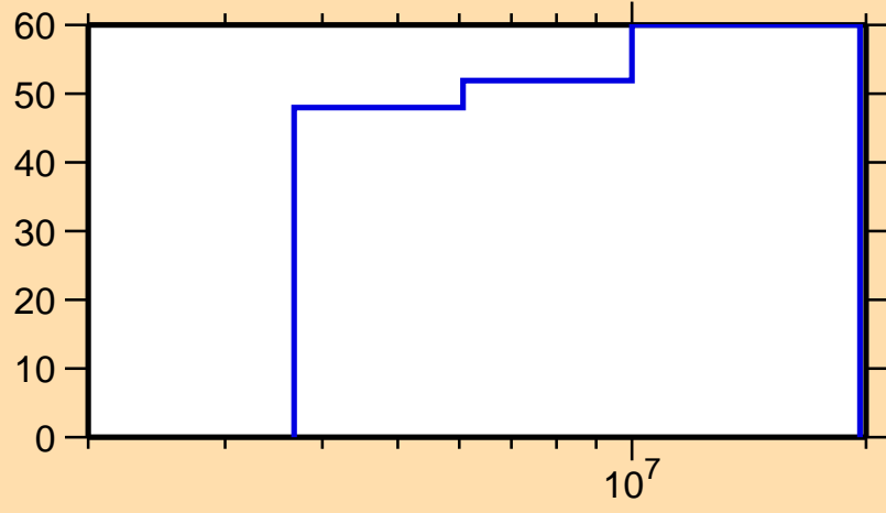
\Delta\sigma/\sigma vs. E for ^{164}\text{Gd}(n,\gamma)
