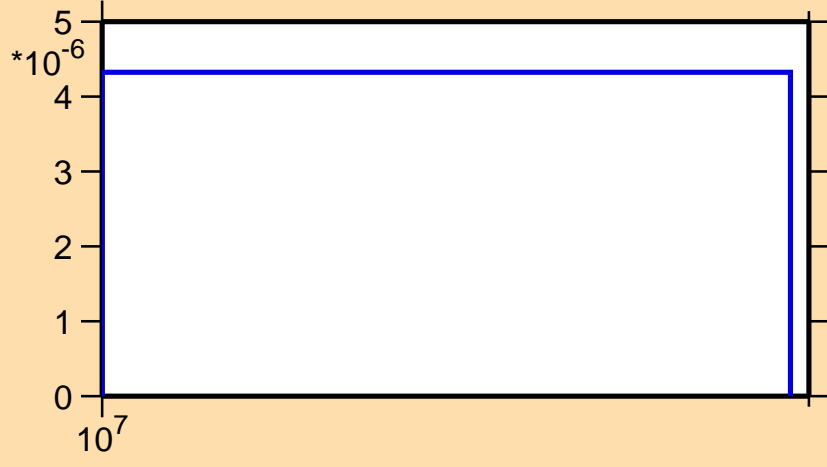
\sigma vs. E for ^{164}\text{Gd}(n,np)
