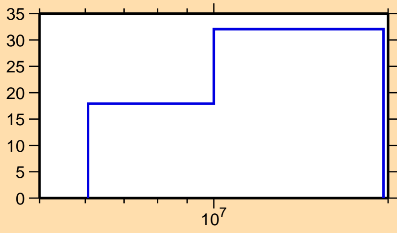
\Delta\sigma/\sigma vs. E for ^{164}\text{Gd}(n,2n)
