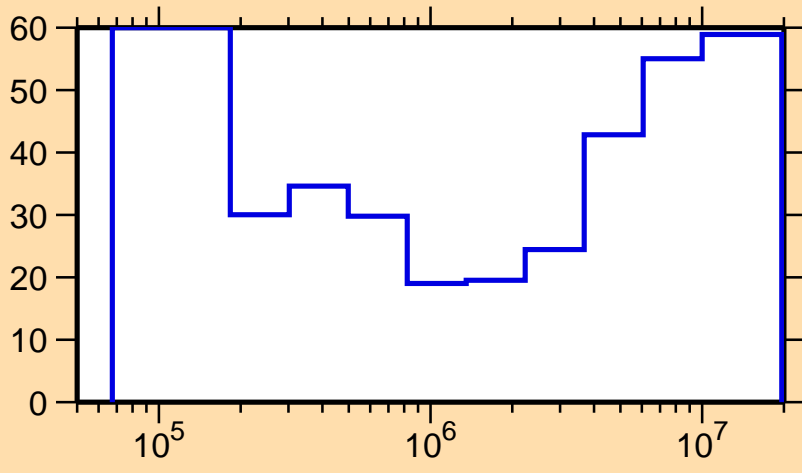
\Delta\sigma/\sigma vs. E for ^{164}\text{Gd}(n,n_1)
