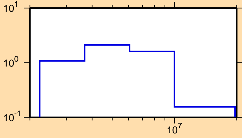
\sigma vs. E for ^{164}\text{Gd}(n,n\text{cont.})
