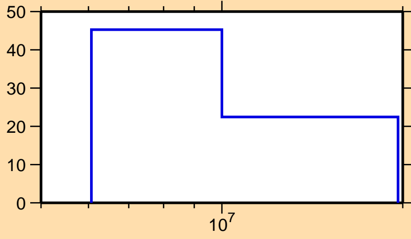
\Delta\sigma/\sigma vs. E for ^{164}\text{Gd}(n,\text{el.})
