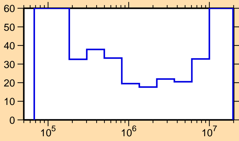
\Delta\sigma/\sigma vs. E for ^{164}\text{Gd}(n,\text{inel.})
