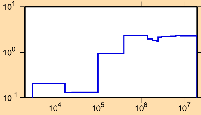
\sigma vs. E for ^{164}\text{Gd}(n,\text{nonel.})
