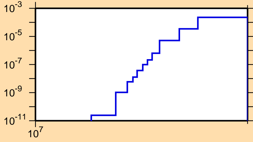
\sigma vs. E for ^{165}\text{Gd}(n,np)
