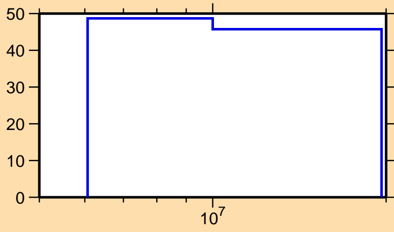
\Delta\sigma/\sigma vs. E for ^{165}\text{Gd}(n,p)
