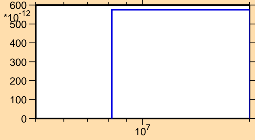
\sigma vs. E for ^{165}\text{Gd}(n,2n\alpha)
