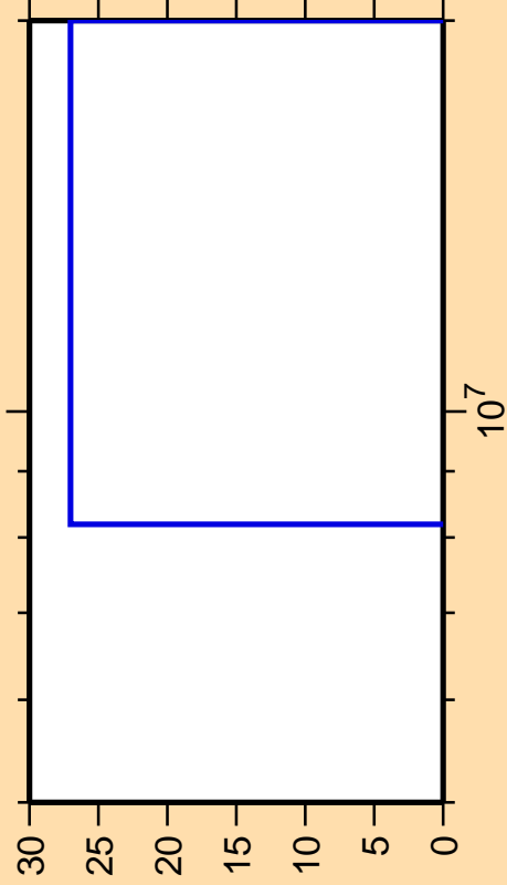
\Delta\sigma/\sigma vs. E for ^{165}\text{Gd}(n,3n)
