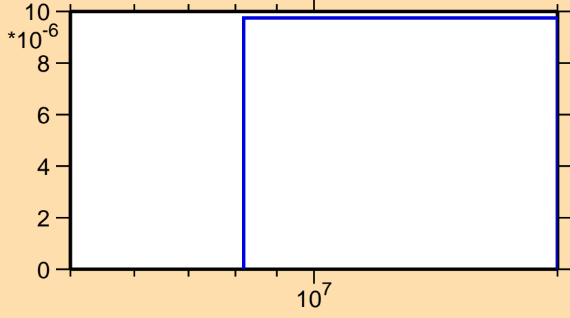
\sigma vs. E for ^{165}\text{Gd}(n,d)
