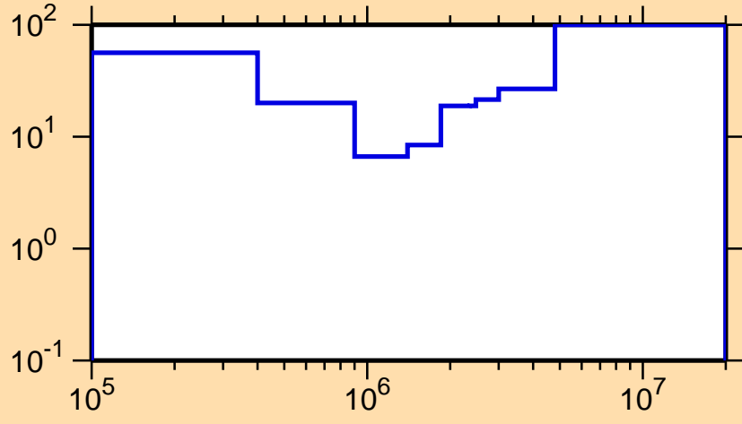
\Delta\sigma/\sigma vs. E for ^{165}\text{Gd}(n,n\text{cont.})
