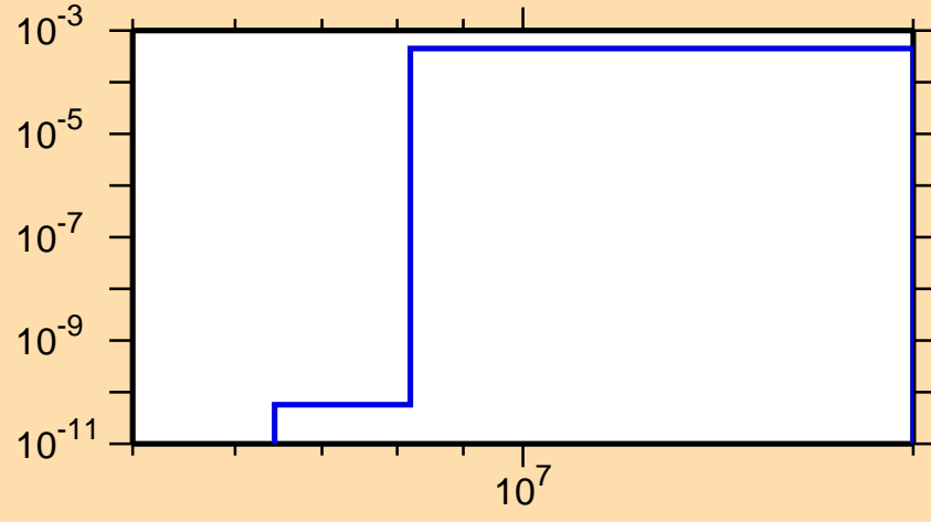
\sigma vs. E for ^{165}\text{Gd}(n,p)
