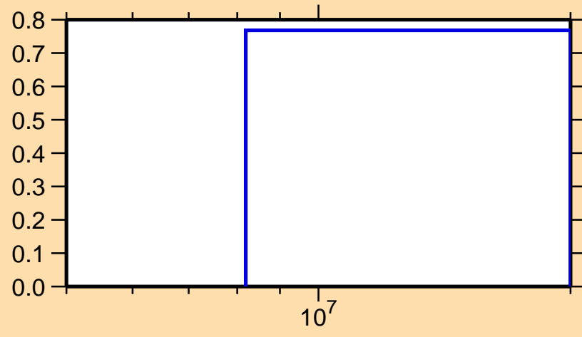
\sigma vs. E for ^{165}\text{Gd}(n,3n)
