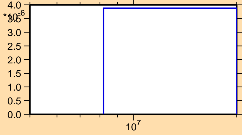
\sigma vs. E for ^{165}\text{Gd}(n,np)
