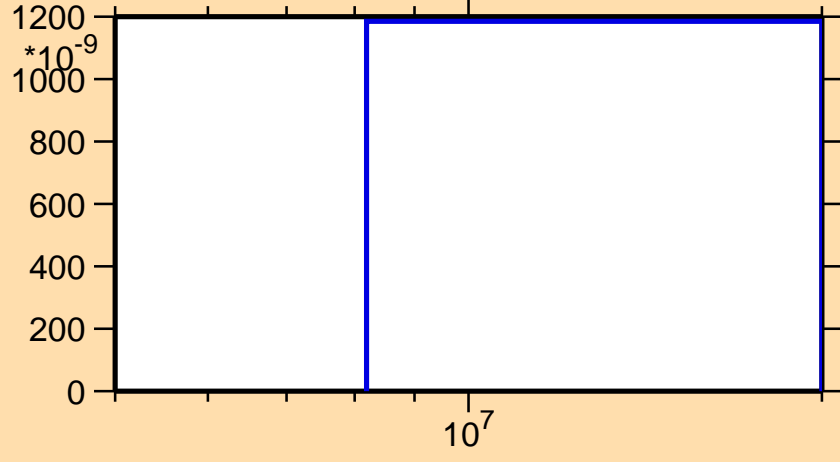
\sigma vs. E for ^{165}\text{Gd}(n,n\alpha)
