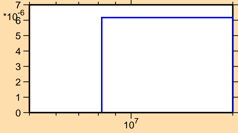
\sigma vs. E for ^{165}\text{Gd}(n,t)
