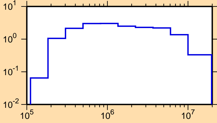
\sigma vs. E for ^{166}\text{Gd}(n,\text{inel.})
