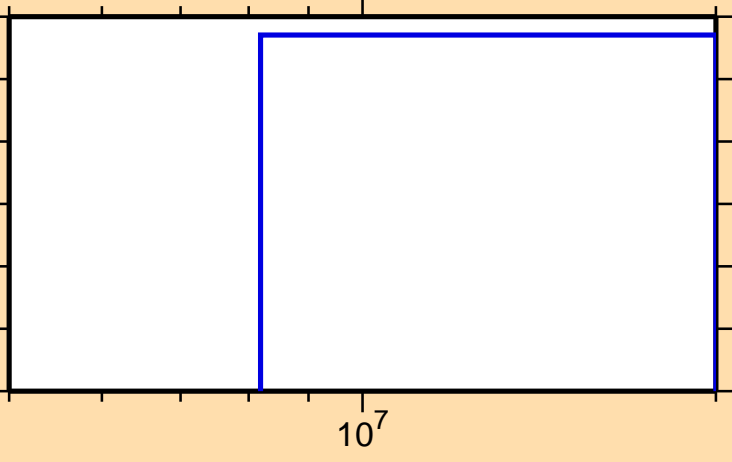
\sigma vs. E for ^{166}\text{Gd}(n,t)
