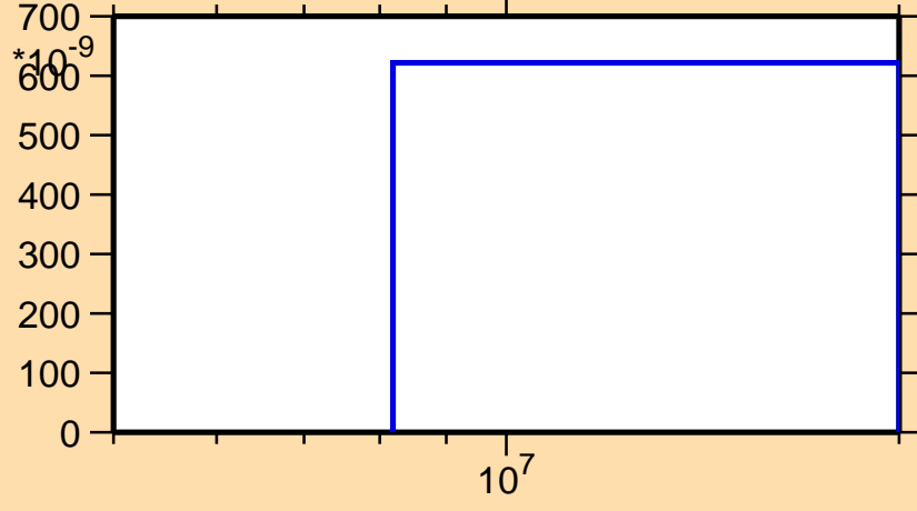
\sigma vs. E for ^{166}\text{Gd}(n,n\alpha)
