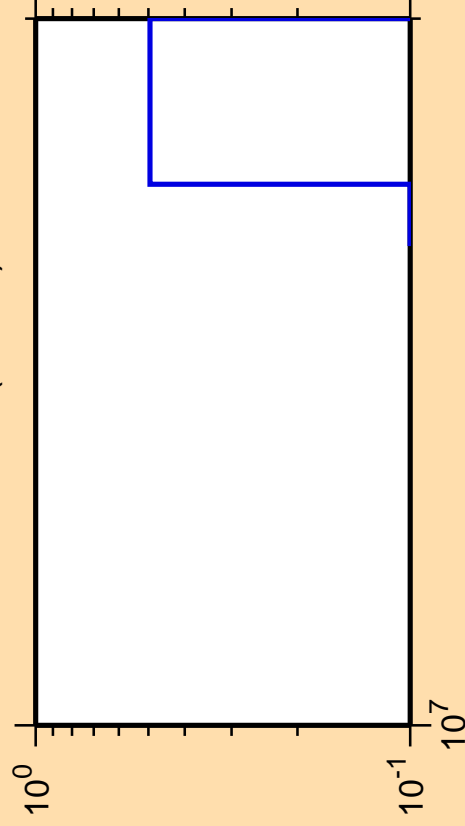
\Delta\sigma/\sigma vs. E for ^{167}\text{Gd}(n,3n\alpha)
