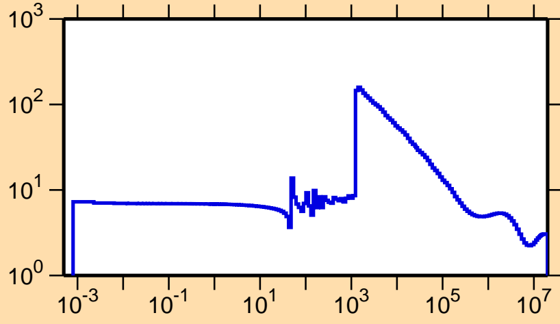
\sigma vs. E for ^{167}\text{Gd}(n,\text{el.})
