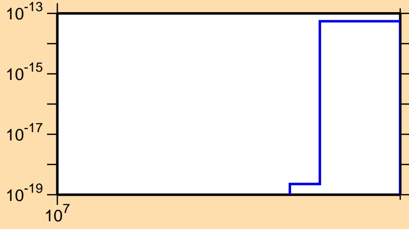
\sigma vs. E for ^{167}\text{Gd}(n,3n\alpha)
