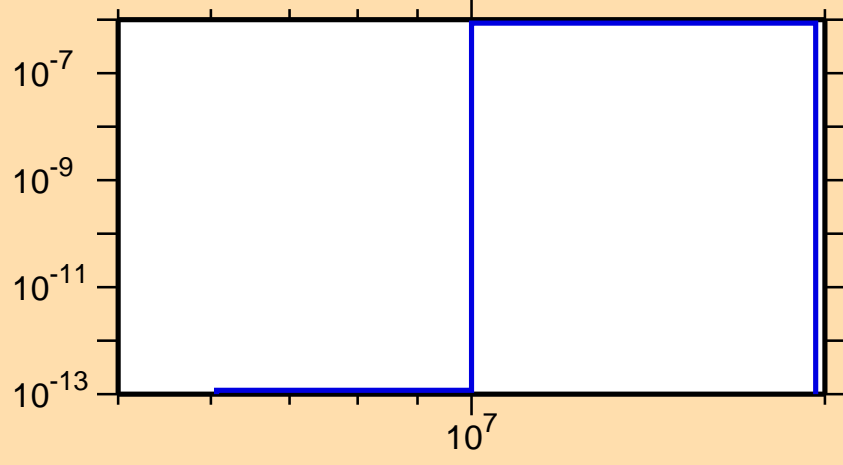
\sigma vs. E for ^{167}\text{Gd}(n,n\alpha)
