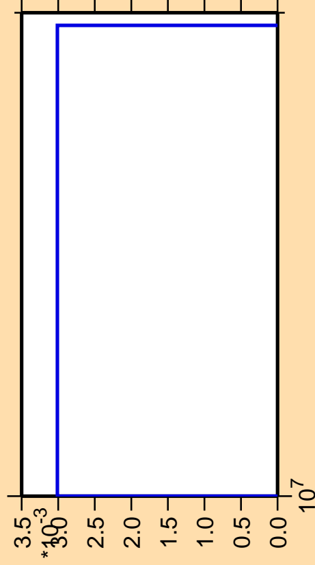
\Delta\sigma/\sigma vs. E for ^{167}\text{Gd}(n,3n\alpha)
