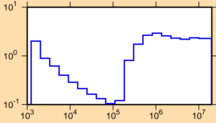
\sigma vs. E for ^{167}\text{Gd}(n,\text{nonel.})
