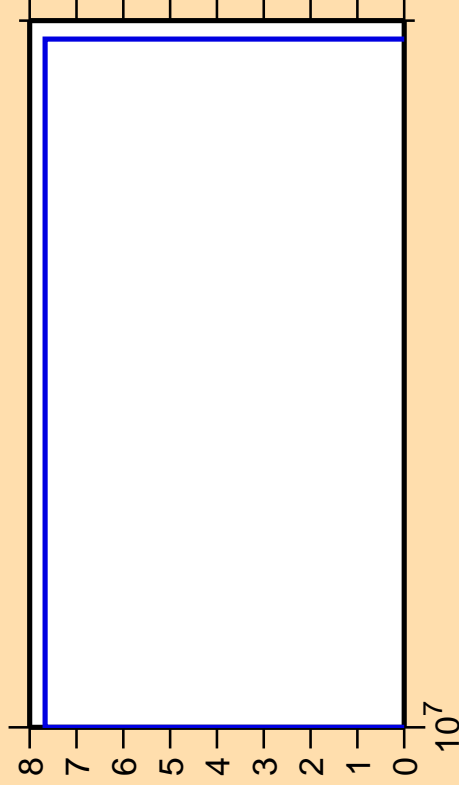
\Delta\sigma/\sigma vs. E for ^{167}\text{Gd}(n,2np)
