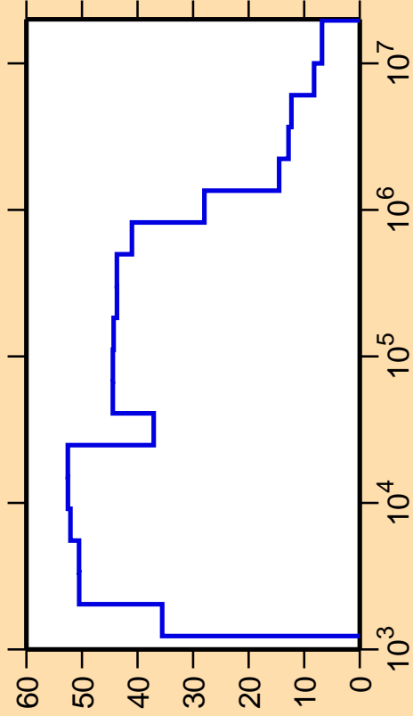
\Delta\sigma/\sigma vs. E for ^{167}\text{Gd}(n,\text{nonel.})
