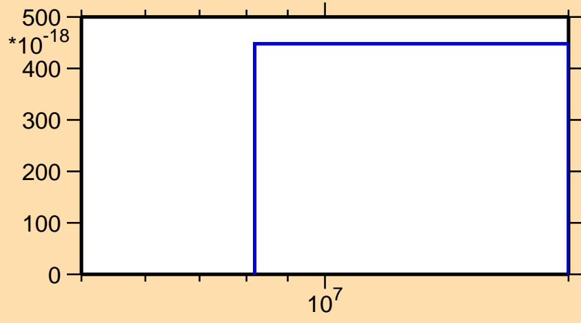
\sigma vs. E for ^{167}\text{Gd}(n,3n\alpha)
