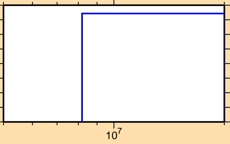
\sigma vs. E for ^{167}\text{Gd}(n,t)
