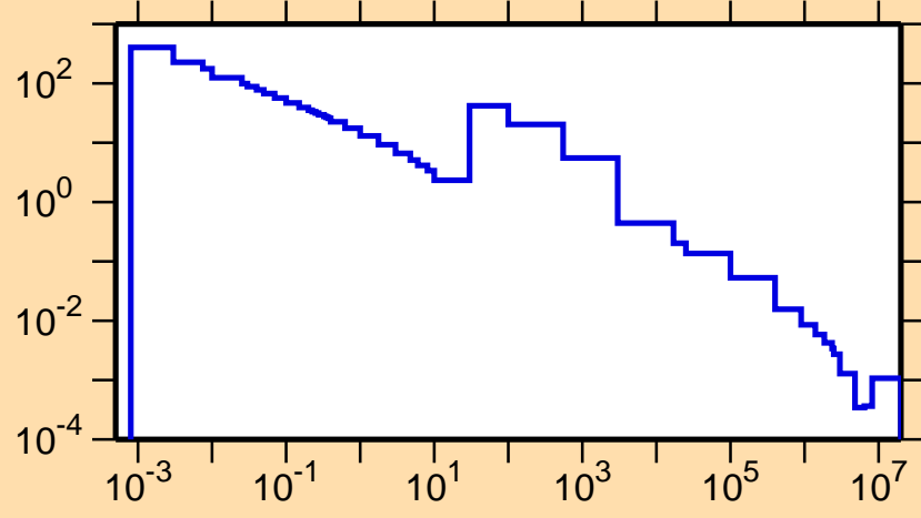
\sigma vs. E for ^{167}\text{Gd}(n,\gamma)
