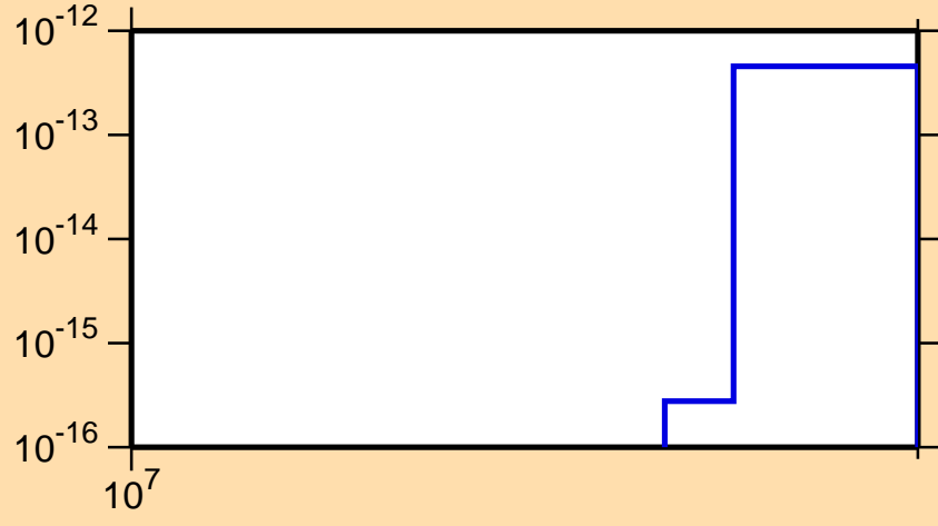
\sigma vs. E for ^{169}\text{Gd}(n,3n\alpha)
