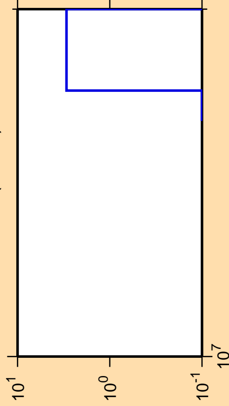
\Delta\sigma/\sigma vs. E for ^{169}\text{Gd}(n,3n\alpha)
