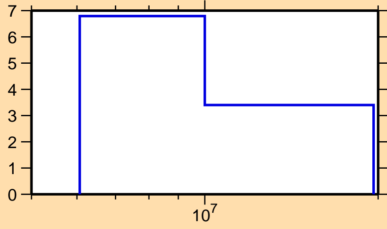
\Delta\sigma/\sigma vs. E for ^{169}\text{Gd}(n,\text{nonel.})
