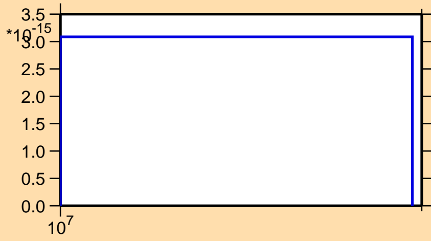
\sigma vs. E for ^{169}\text{Gd}(n,3n\alpha)
