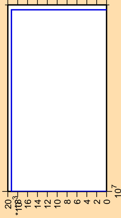
\Delta\sigma/\sigma vs. E for ^{169}\text{Gd}(n,3n\alpha)
