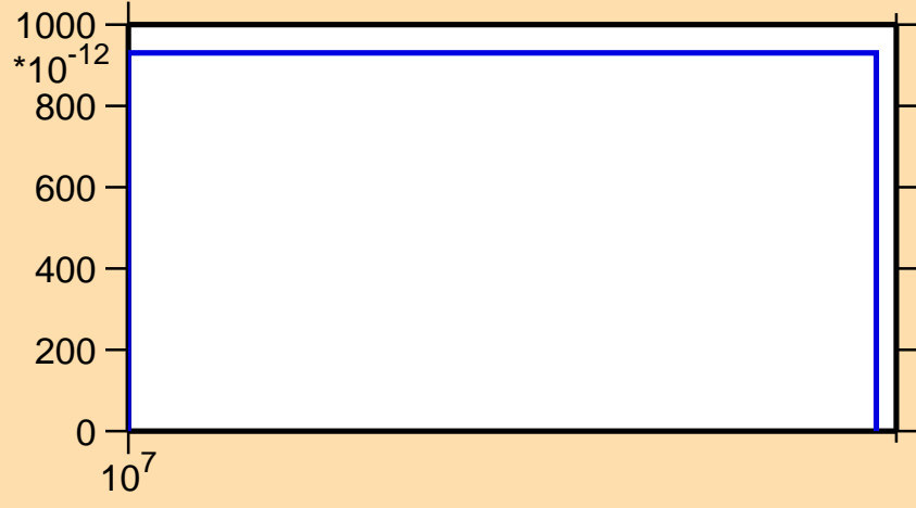
\sigma vs. E for ^{169}\text{Gd}(n,nd)
