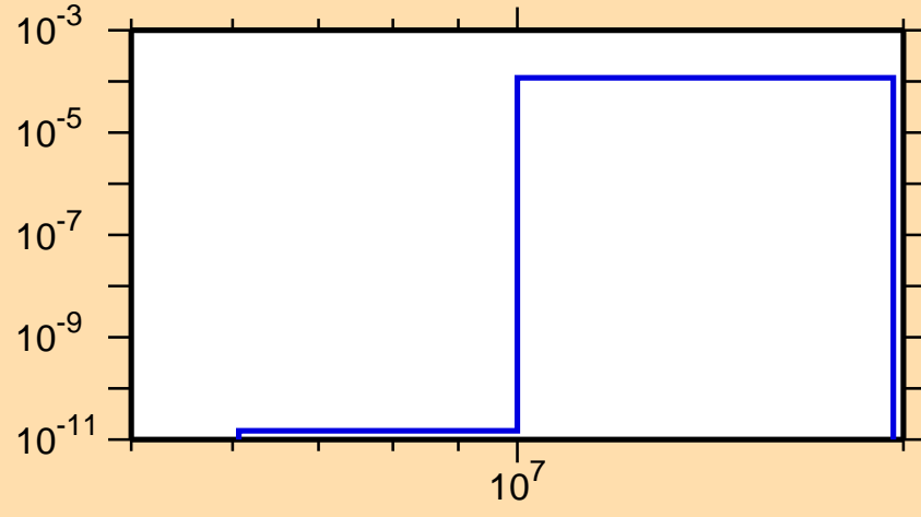
\sigma vs. E for ^{169}\text{Gd}(n,p)
