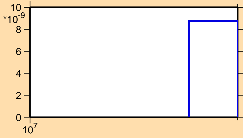
\sigma vs. E for ^{64}\text{Ge}(n,2np)
