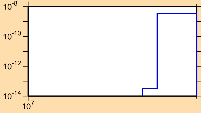
\sigma vs. E for ^{64}\text{Ge}(n,\text{nd})
