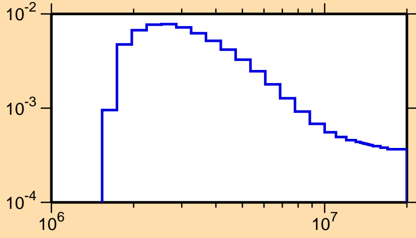
\sigma vs. E for ^{64}\text{Ge}(n,n_2)
