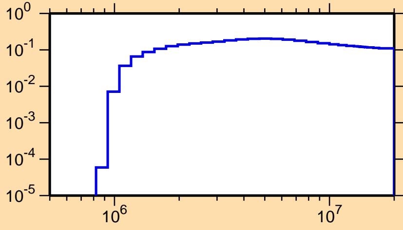
\sigma vs. E for ^{64}\text{Ge}(n,\text{inel.})
