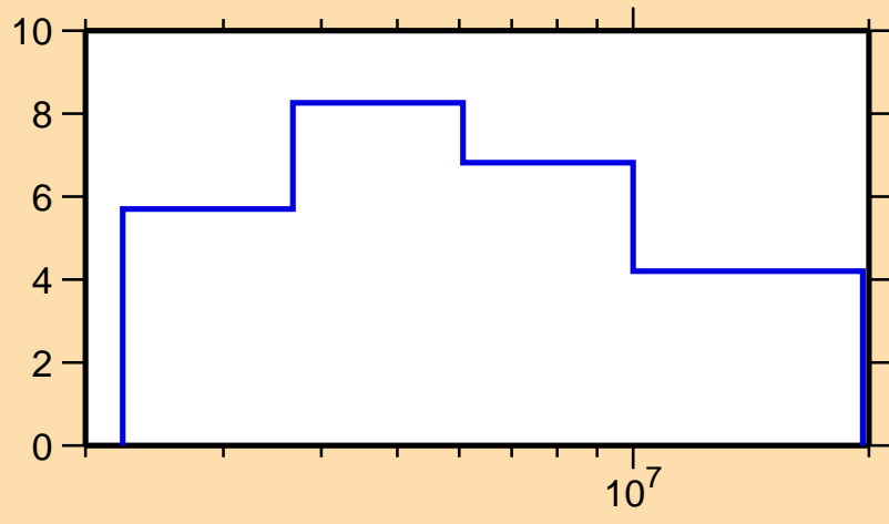
\Delta\sigma/\sigma vs. E for ^{64}\text{Ge}(n,n\text{nonel.})
