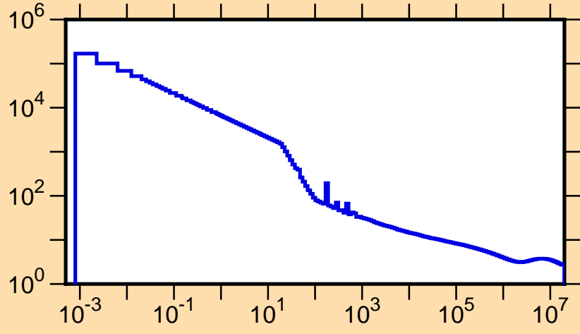
\sigma vs. E for ^{65}\text{Ge}(n,\text{tot.})
