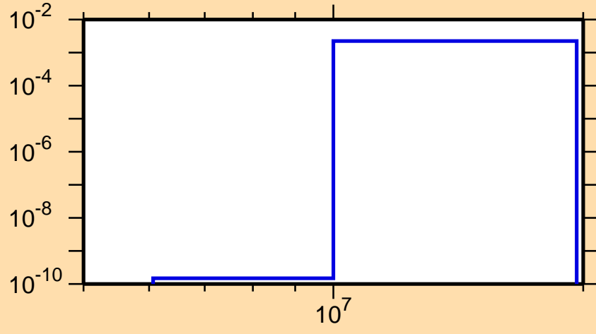
\sigma vs. E for ^{65}\text{Ge}(n,\text{pd})
