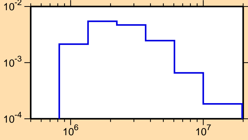
\sigma vs. E for ^{65}\text{Ge}(n,n_4)
