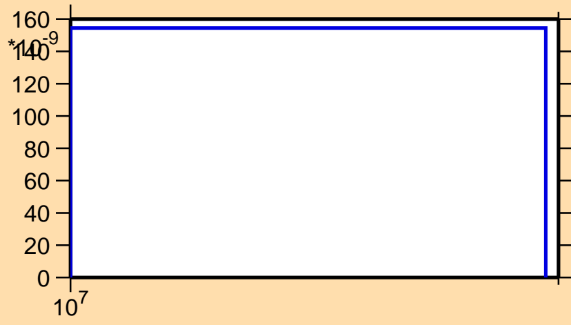
\sigma vs. E for ^{65}\text{Ge}(n,2np)
