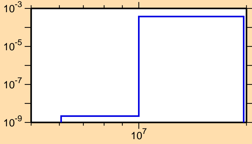
\sigma vs. E for ^{65}\text{Ge}(n,t)
