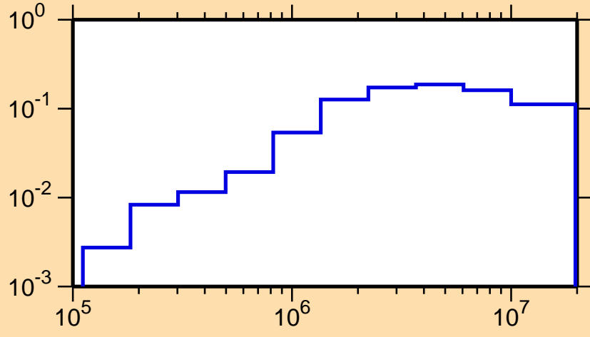
\sigma vs. E for ^{65}\text{Ge}(n,\text{inel.})
