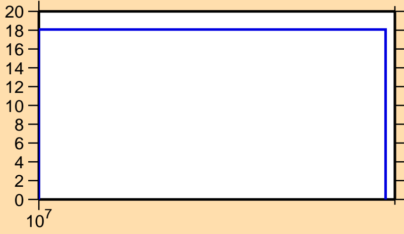
\Delta\sigma/\sigma vs. E for ^{65}\text{Ge}(n,\text{el.})
