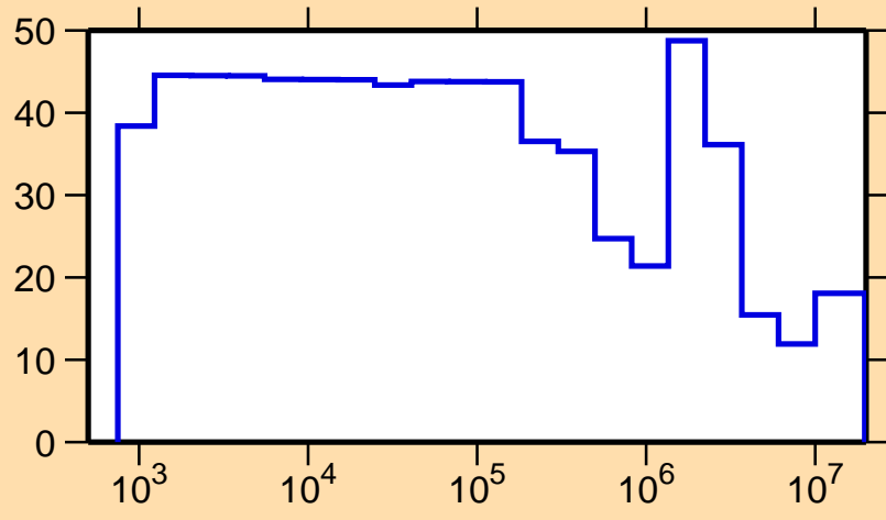
\Delta\sigma/\sigma vs. E for ^{65}\text{Ge}(n,el.)
