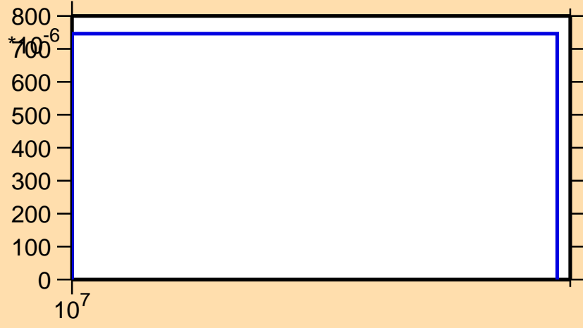
\sigma vs. E for ^{65}\text{Ge}(n,2n)
