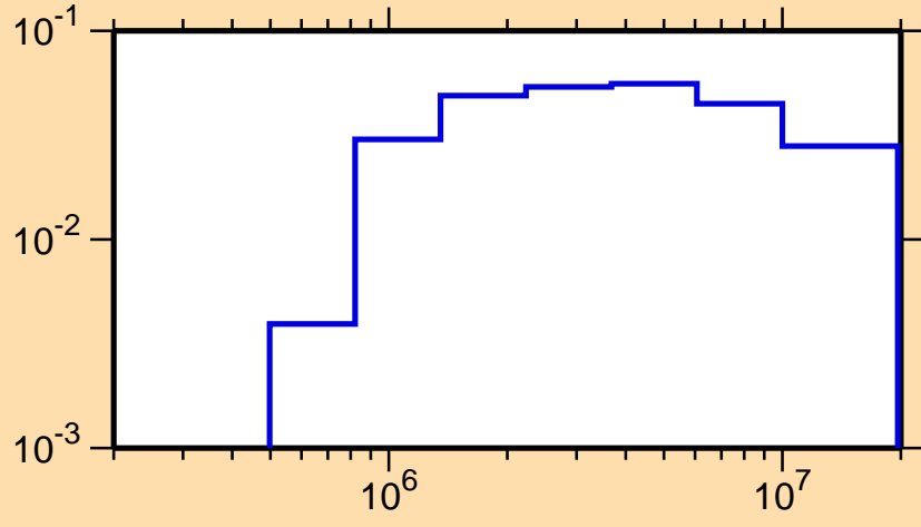
\sigma vs. E for ^{65}\text{Ge}(n,n_2)
