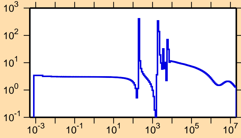
\sigma vs. E for ^{66}\text{Ge}(n,\text{el.})
