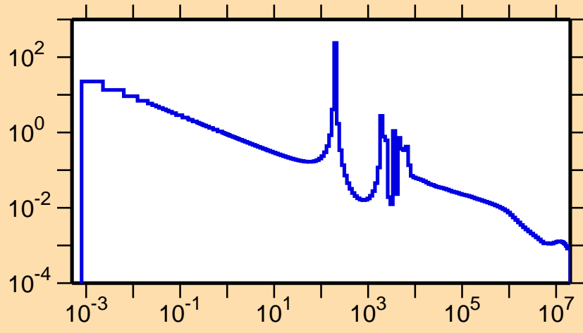
\sigma vs. E for ^{66}\text{Ge}(n,\gamma)
