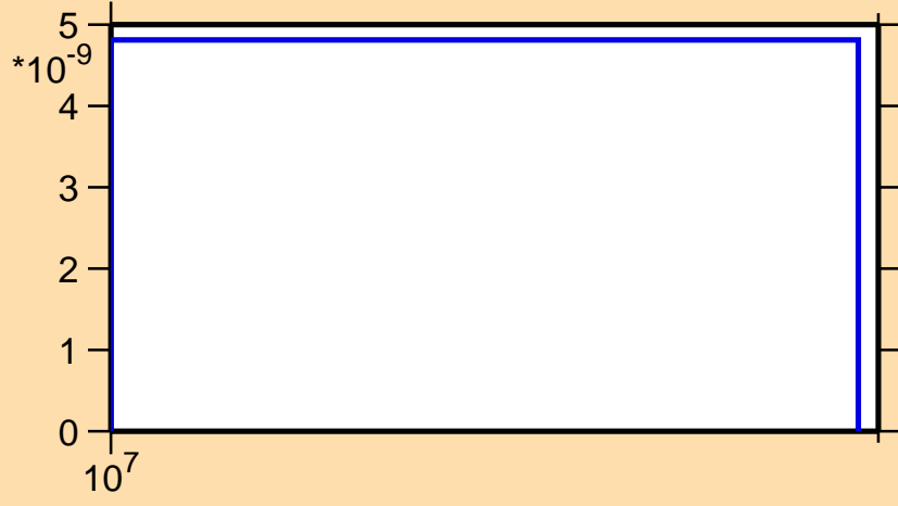
\sigma vs. E for ^{66}\text{Ge}(n,\text{pt})
