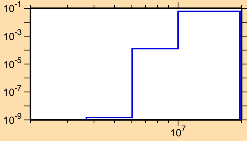
\sigma vs. E for ^{66}\text{Ge}(n,p\alpha)
