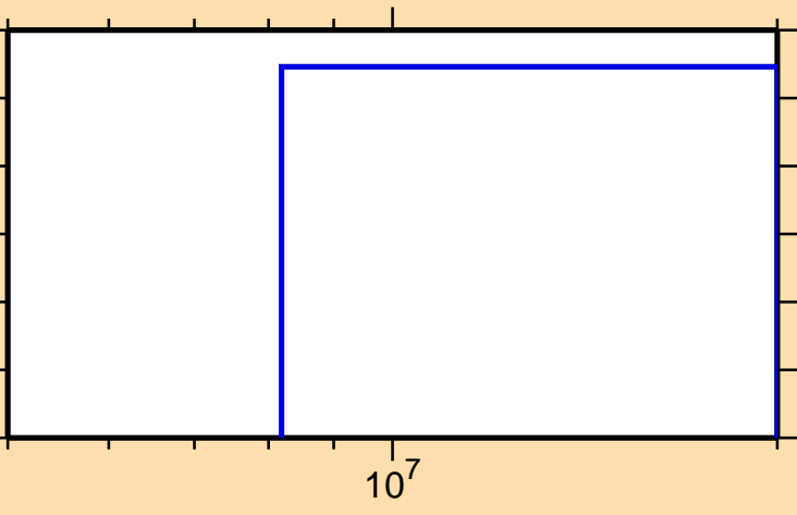
\sigma vs. E for ^{66}\text{Ge}(n,\text{pt})
