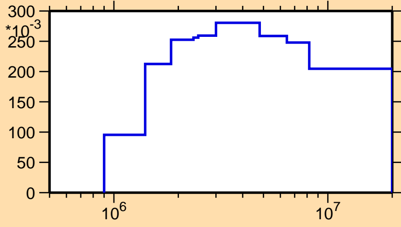
\sigma vs. E for ^{66}\text{Ge}(n,\text{inel.})
