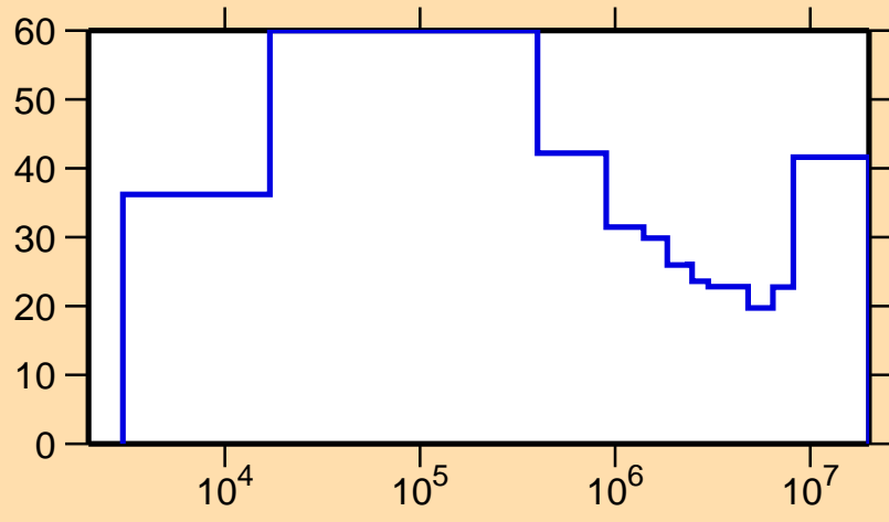
\Delta\sigma/\sigma vs. E for ^{66}\text{Ge}(n,p)
