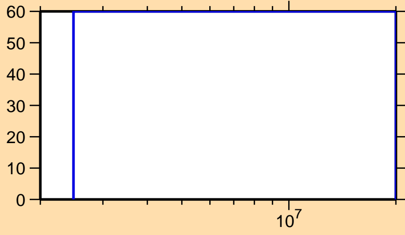
\Delta\sigma/\sigma vs. E for ^{66}\text{Ge}(n,n\text{cont.})
