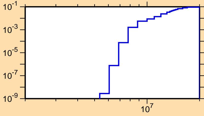
\sigma vs. E for ^{67}\text{Ge}(n,n\alpha)
