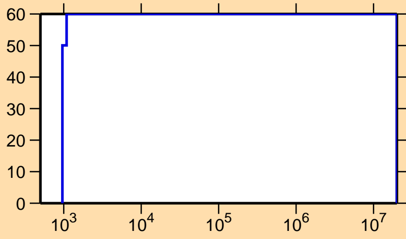
\Delta\sigma/\sigma vs. E for ^{67}\text{Ge}(n,\gamma)
