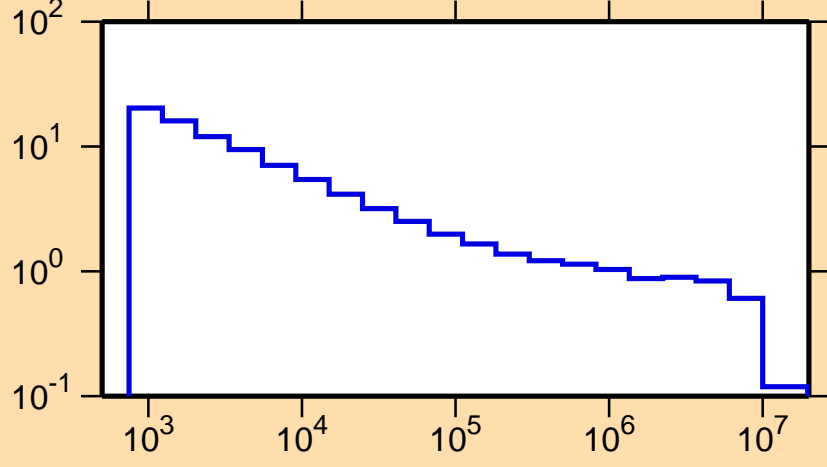
\sigma vs. E for ^{67}\text{Ge}(n,p)
