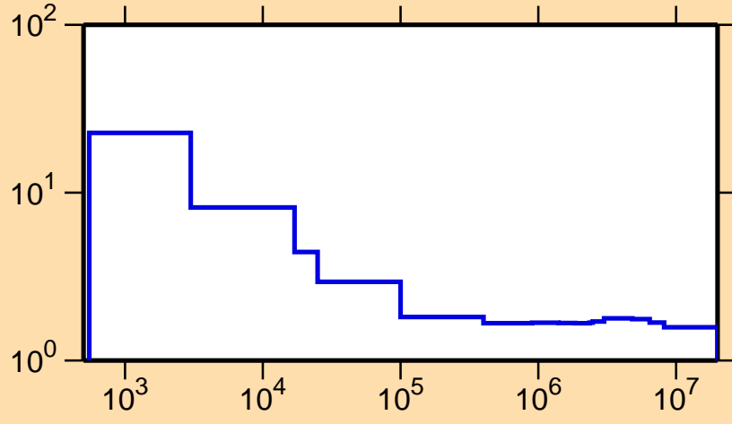
\sigma vs. E for ^{67}\text{Ge}(n,\text{nonel.})
