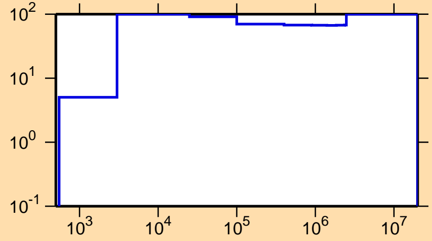
\Delta\sigma/\sigma vs. E for ^{67}\text{Ge}(n,\gamma)
