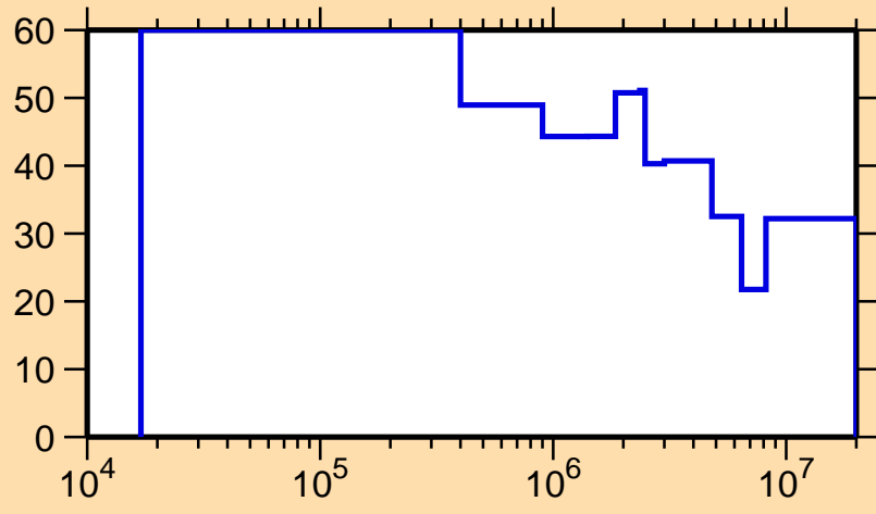
\Delta\sigma/\sigma vs. E for ^{67}\text{Ge}(n,n_1)
