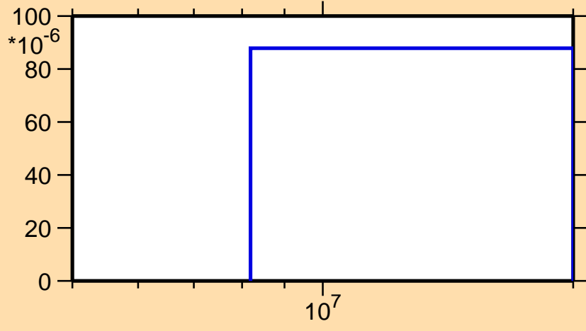
\sigma vs. E for ^{67}\text{Ge}(n,\text{pd})
