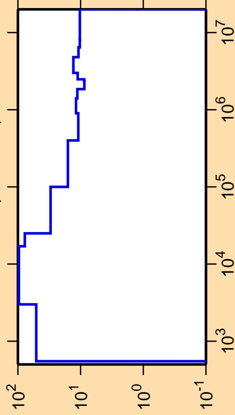
\Delta\sigma/\sigma vs. E for ^{67}\text{Ge}(n,\text{nonel.})
