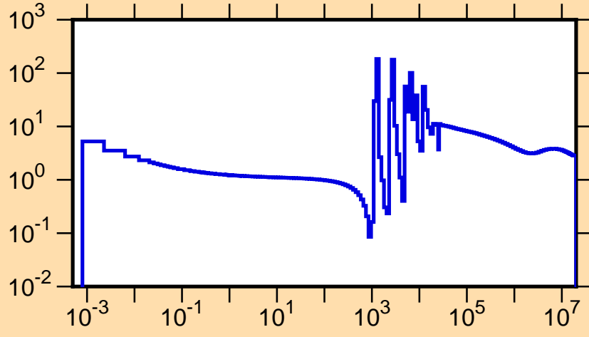
\sigma vs. E for ^{68}\text{Ge}(n,\text{tot.})
