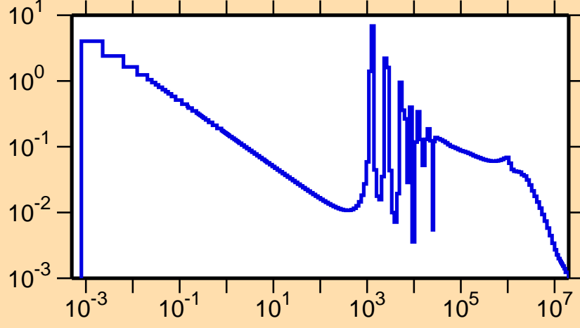
\sigma vs. E for ^{68}\text{Ge}(n,\gamma)
